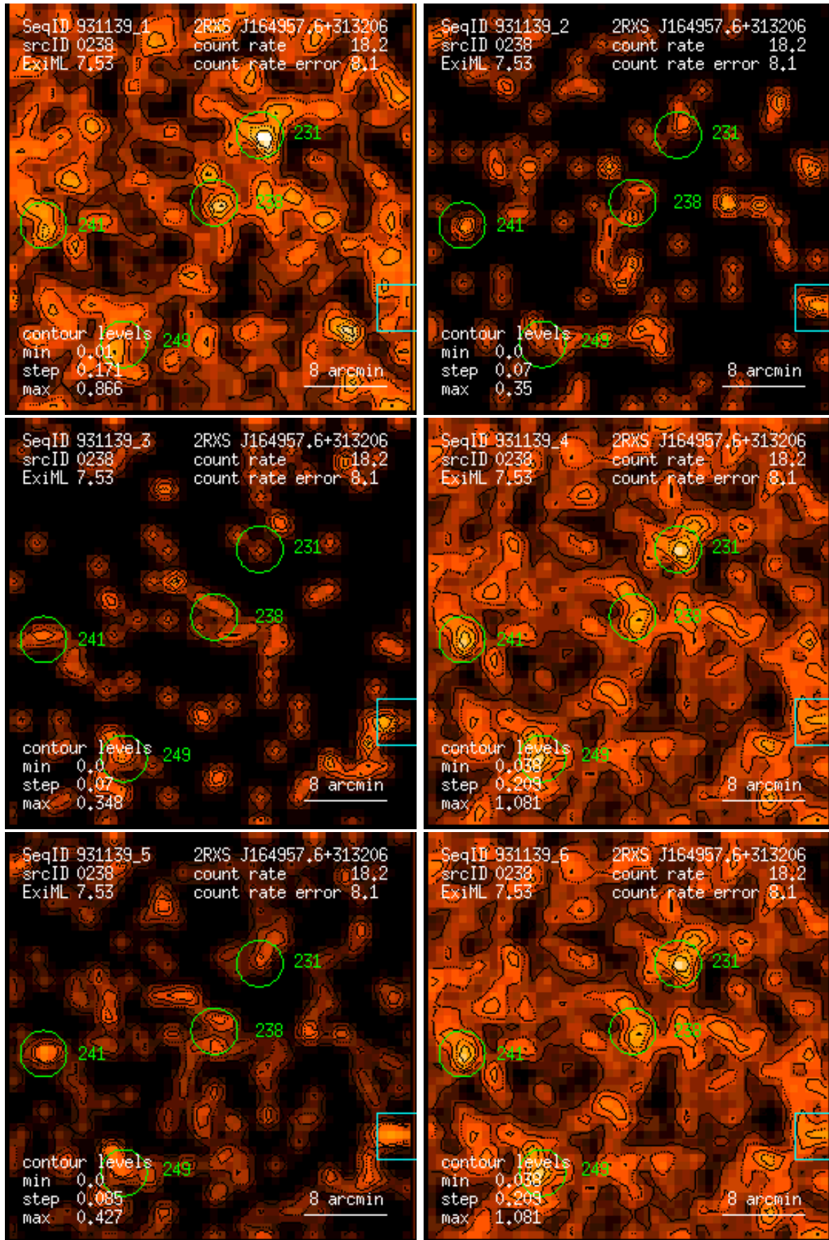
Figure 238: RASS 931139: detection 0238: band rate images, Gaussian filter: (1) PSPC channels 11 – 41, (2) 52 – 90, (3) 91 – 201, (4) 11 – 235, (5) 52 – 201, (6) 11 – 201. Broad band rates in counts/ks. Band rate contour levels in counts/ks/arcmin 2 .
