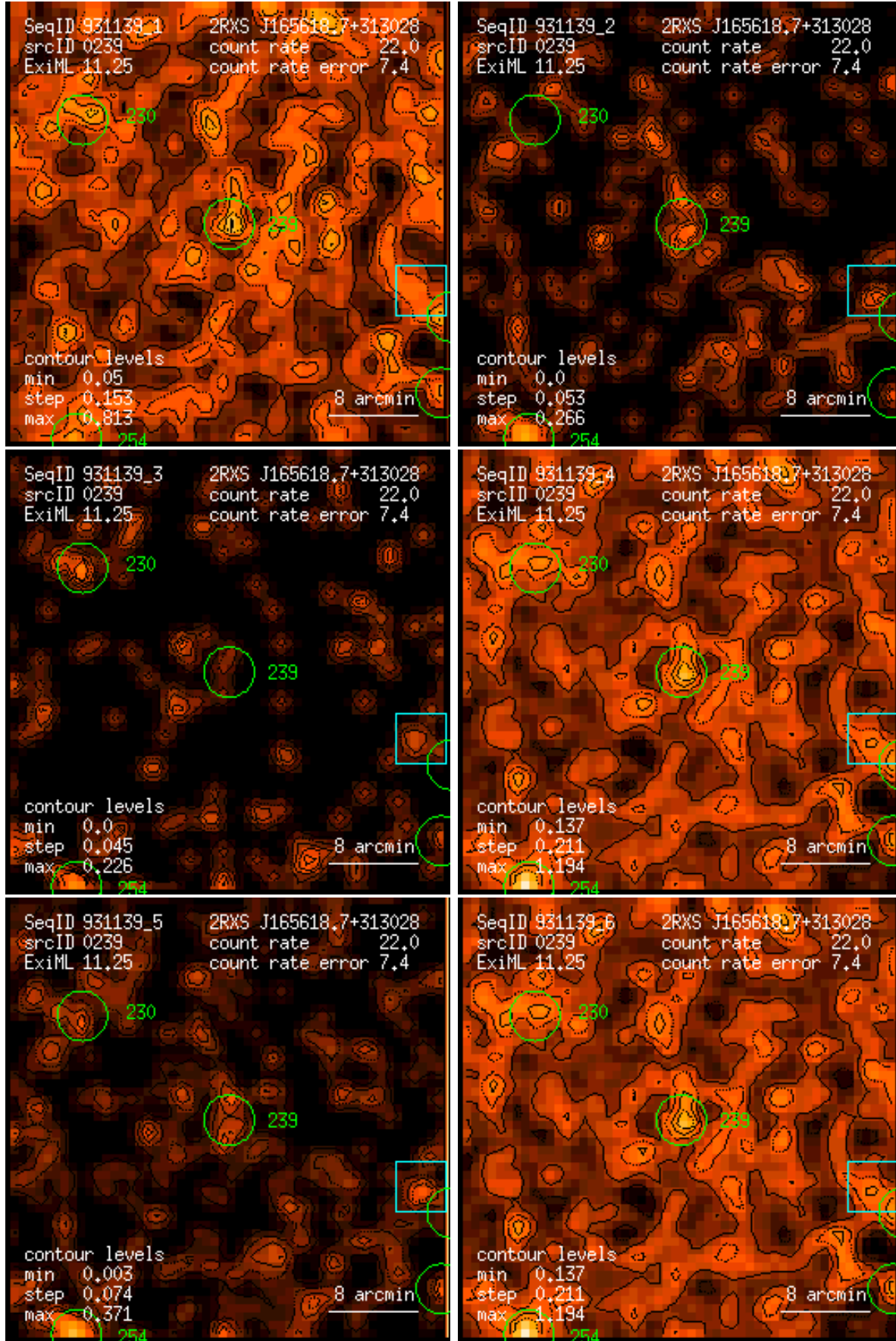
Figure 239: RASS 931139: detection 0239: band rate images, Gaussian filter: (1) PSPC channels 11 – 41, (2) 52 – 90, (3) 91 – 201, (4) 11 – 235, (5) 52 – 201, (6) 11 – 201. Broad band rates in counts/ks. Band rate contour levels in counts/ks/arcmin 2 .
