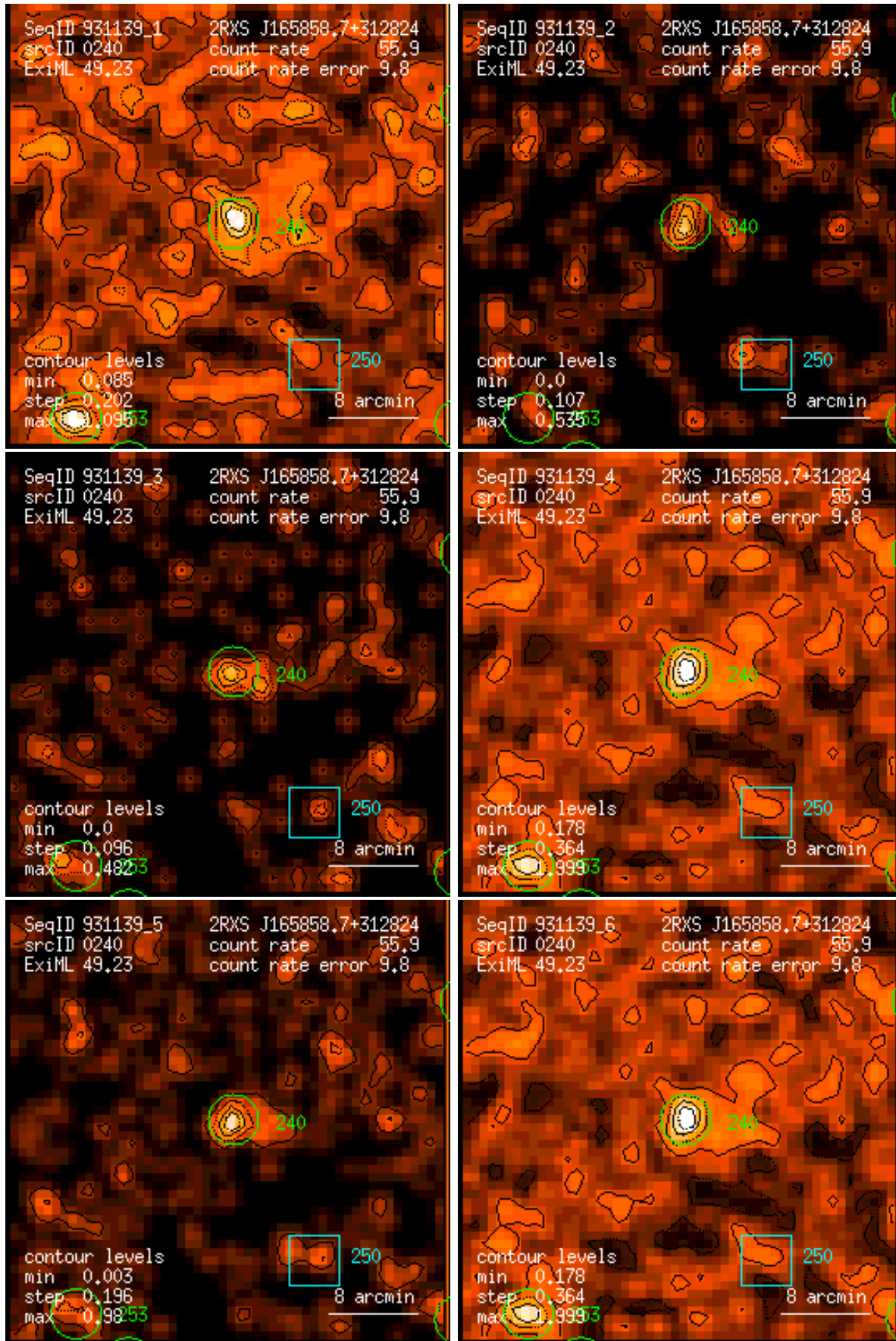
Figure 240: RASS 931139: detection 0240: band rate images, Gaussian filter: (1) PSPC channels 11 – 41, (2) 52 – 90, (3) 91 – 201, (4) 11 – 235, (5) 52 – 201, (6) 11 – 201. Broad band rates in counts/ks. Band rate contour levels in counts/ks/arcmin 2 .
