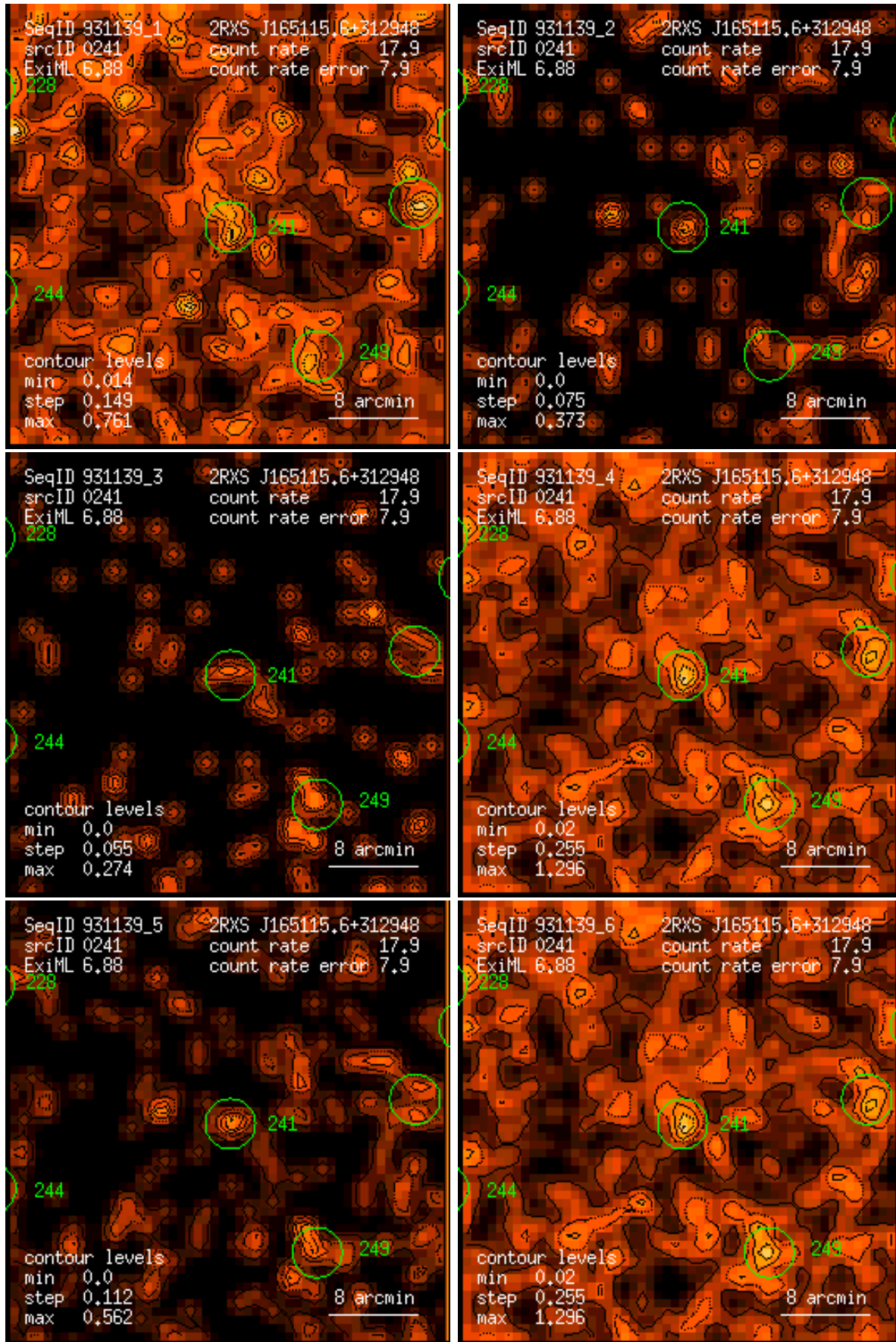
Figure 241: RASS 931139: detection 0241: band rate images, Gaussian filter: (1) PSPC channels 11 – 41, (2) 52 – 90, (3) 91 – 201, (4) 11 – 235, (5) 52 – 201, (6) 11 – 201. Broad band rates in counts/ks. Band rate contour levels in counts/ks/arcmin 2 .
