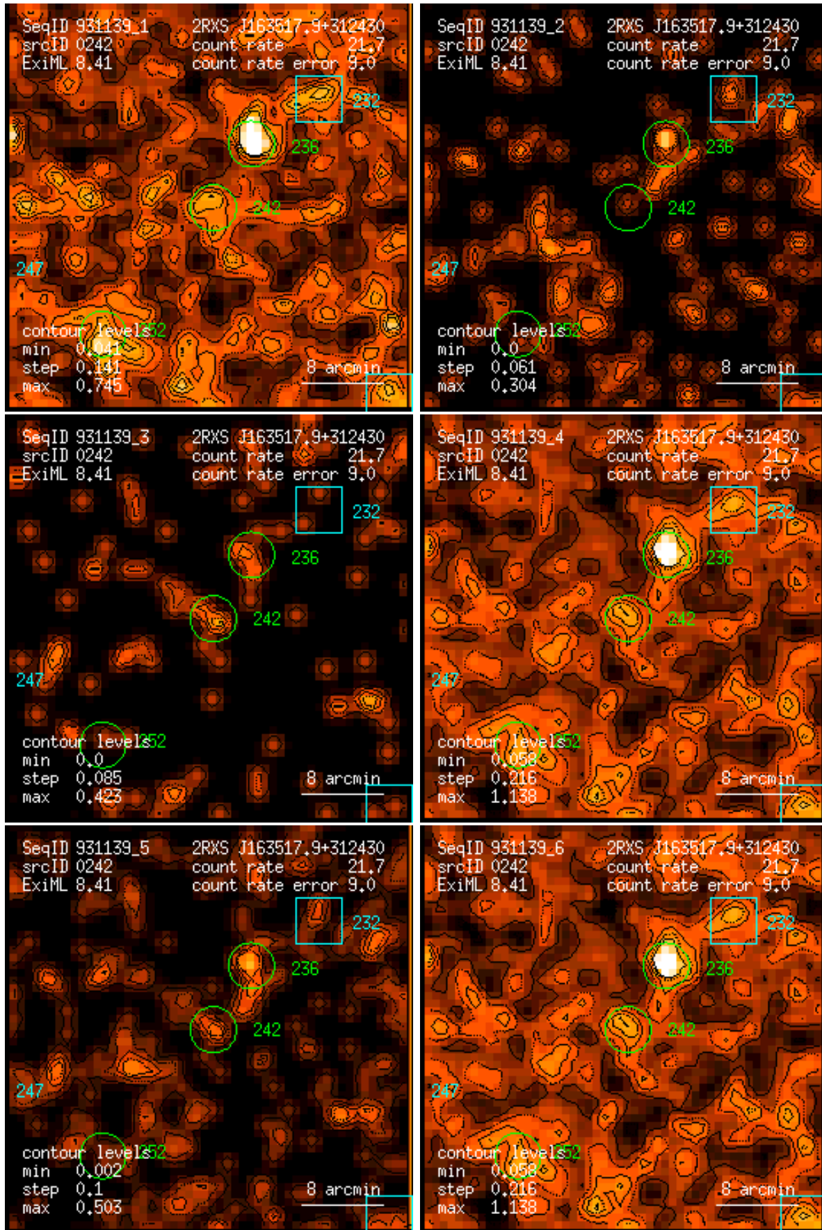
Figure 242: RASS 931139: detection 0242: band rate images, Gaussian filter: (1) PSPC channels 11 – 41, (2) 52 – 90, (3) 91 – 201, (4) 11 – 235, (5) 52 – 201, (6) 11 – 201. Broad band rates in counts/ks. Band rate contour levels in counts/ks/arcmin 2 .
