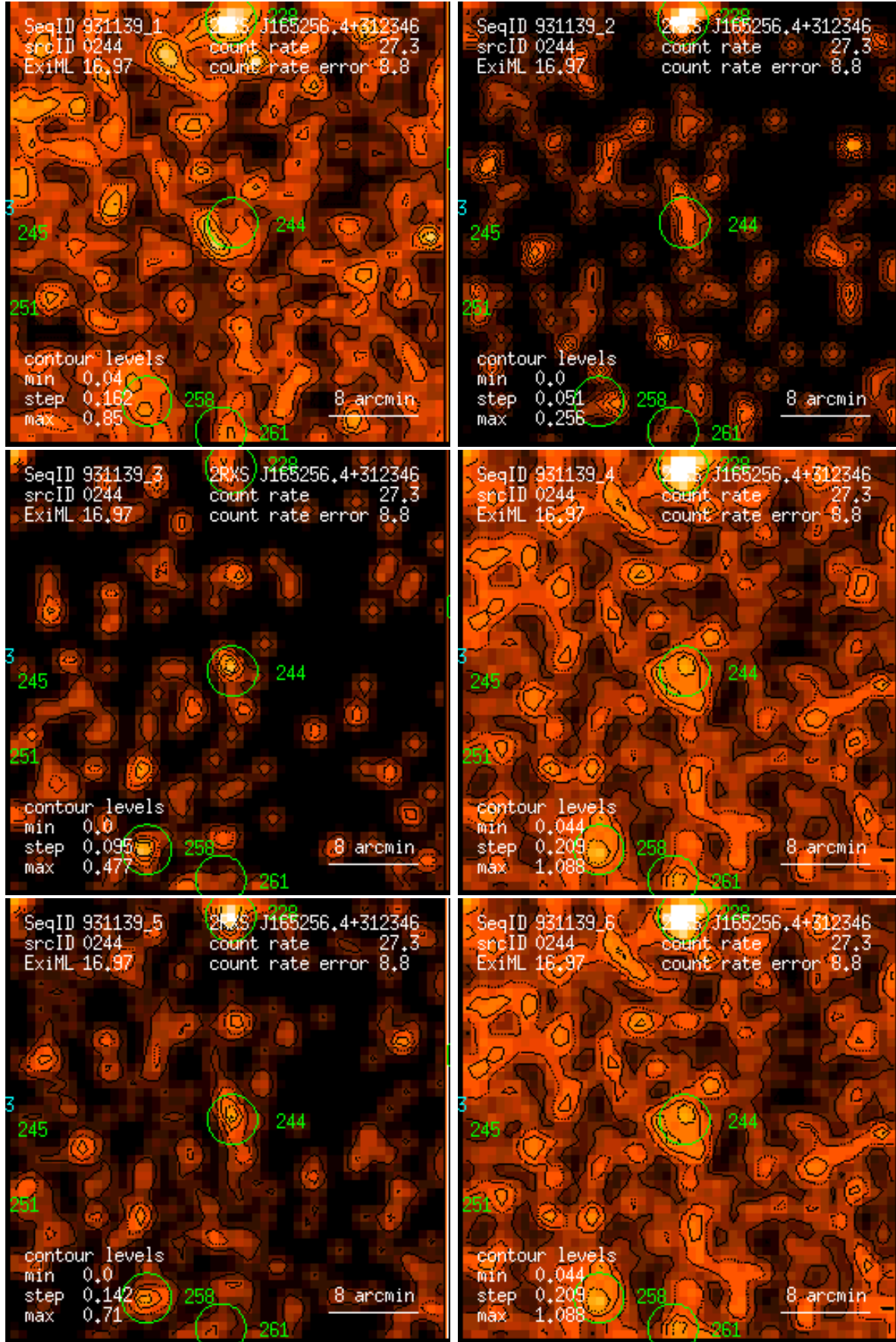
Figure 244: RASS 931139: detection 0244: band rate images, Gaussian filter: (1) PSPC channels 11 – 41, (2) 52 – 90, (3) 91 – 201, (4) 11 – 235, (5) 52 – 201, (6) 11 – 201. Broad band rates in counts/ks. Band rate contour levels in counts/ks/arcmin 2 .
