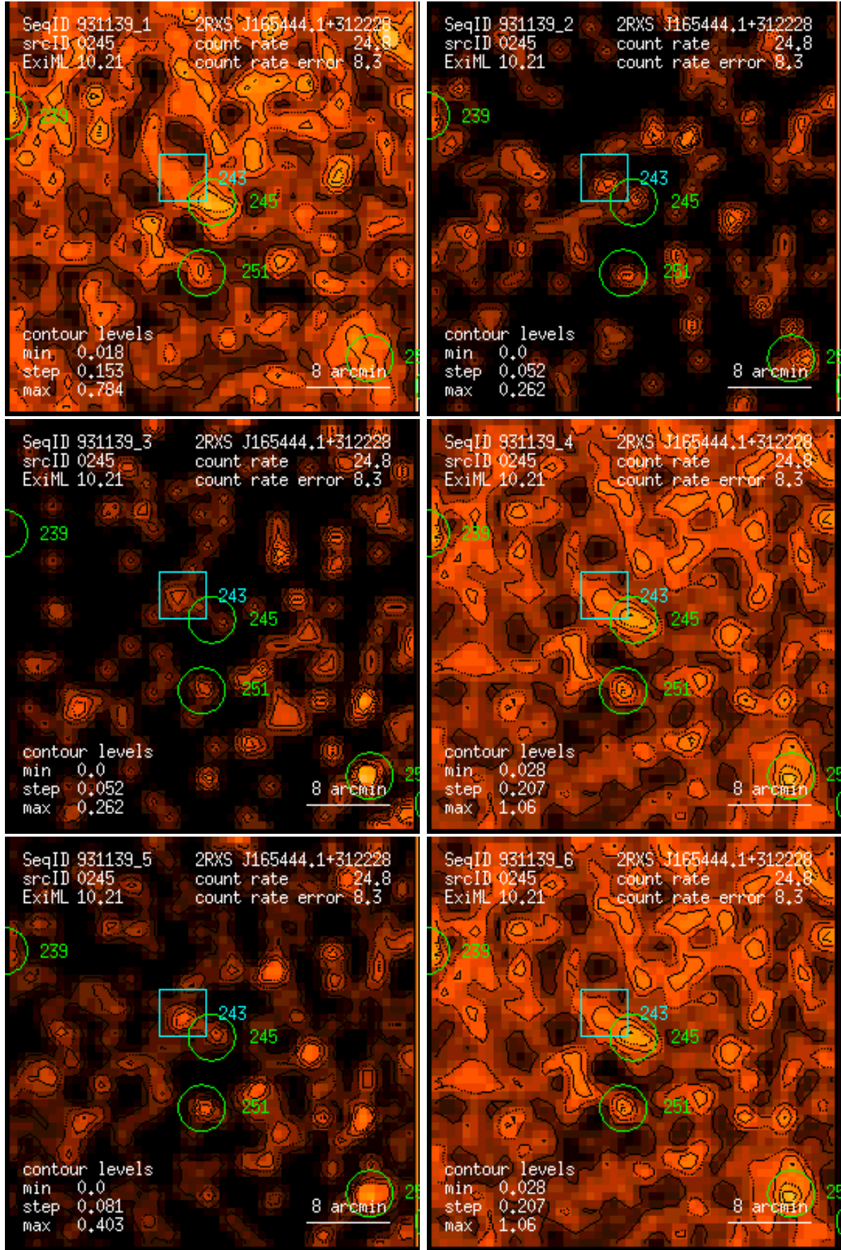
Figure 245: RASS 931139: detection 0245: band rate images, Gaussian filter: (1) PSPC channels 11 – 41, (2) 52 – 90, (3) 91 – 201, (4) 11 – 235, (5) 52 – 201, (6) 11 – 201. Broad band rates in counts/ks. Band rate contour levels in counts/ks/arcmin 2 .
