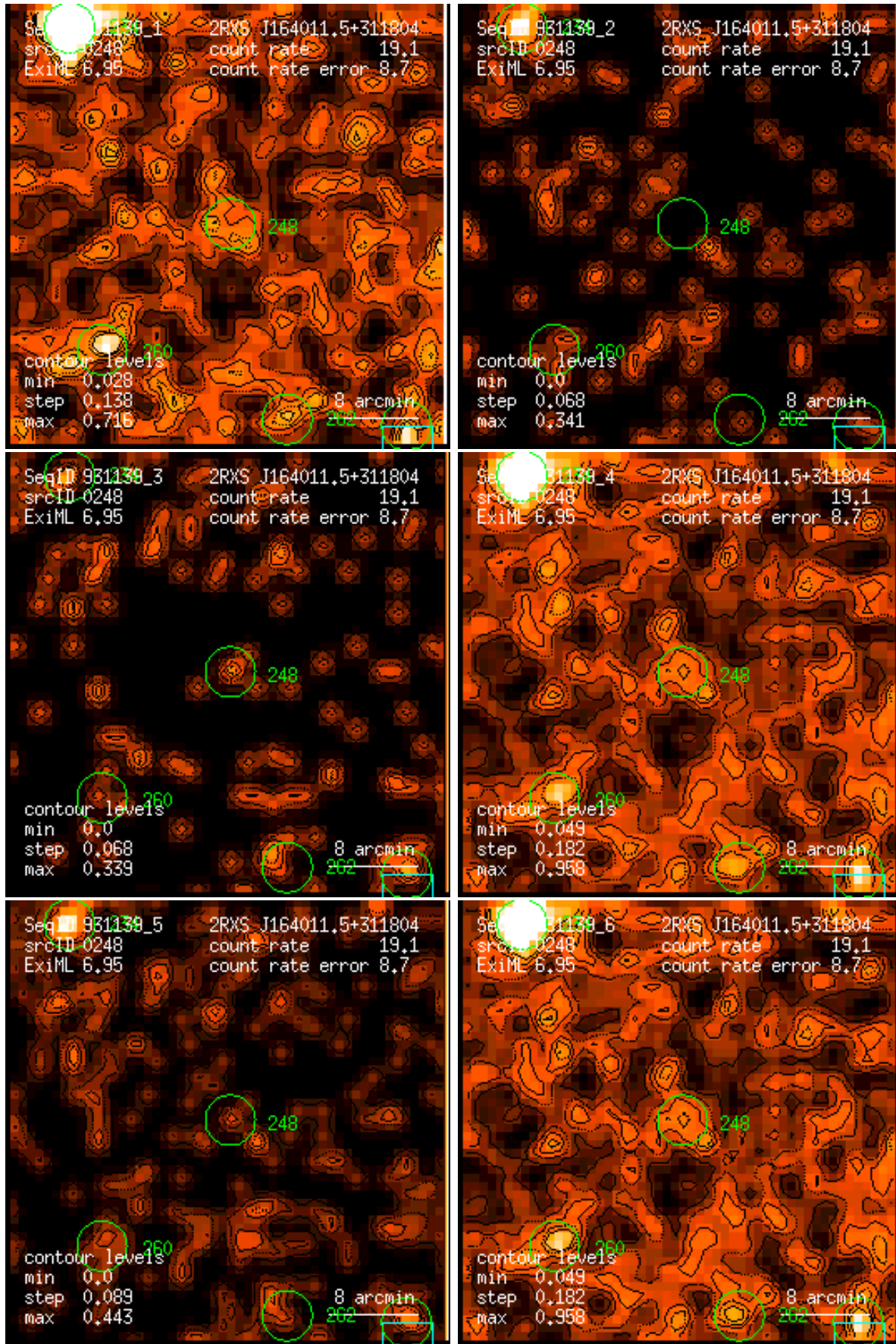
Figure 248: RASS 931139: detection 0248: band rate images, Gaussian filter: (1) PSPC channels 11 – 41, (2) 52 – 90, (3) 91 – 201, (4) 11 – 235, (5) 52 – 201, (6) 11 – 201. Broad band rates in counts/ks. Band rate contour levels in counts/ks/arcmin 2 .
