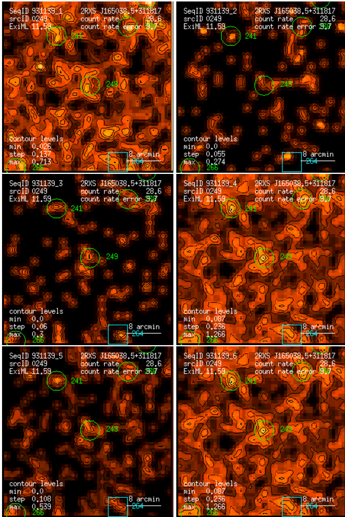
Figure 249: RASS 931139: detection 0249: band rate images, Gaussian filter: (1) PSPC channels 11 – 41, (2) 52 – 90, (3) 91 – 201, (4) 11 – 235, (5) 52 – 201, (6) 11 – 201. Broad band rates in counts/ks. Band rate contour levels in counts/ks/arcmin 2 .
