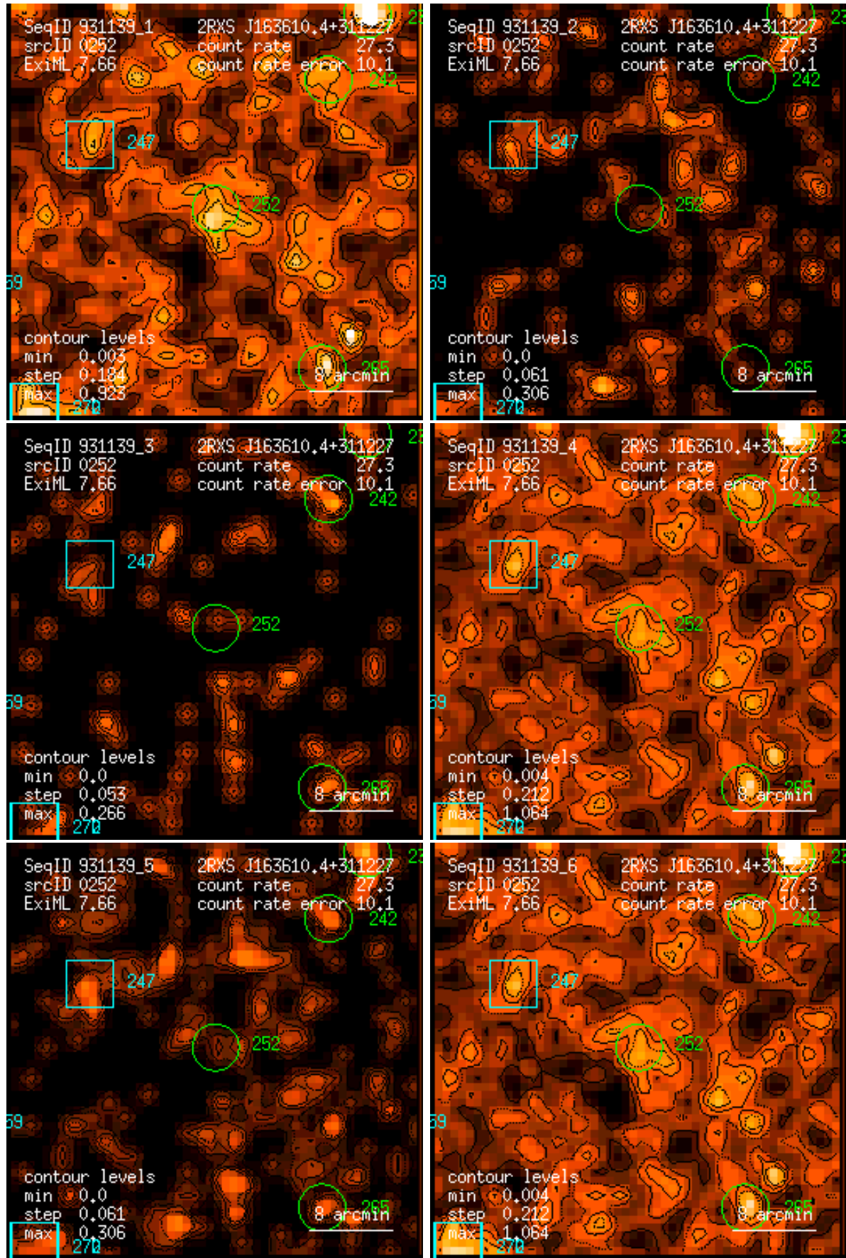
Figure 252: RASS 931139: detection 0252: band rate images, Gaussian filter: (1) PSPC channels 11 – 41, (2) 52 – 90, (3) 91 – 201, (4) 11 – 235, (5) 52 – 201, (6) 11 – 201. Broad band rates in counts/ks. Band rate contour levels in counts/ks/arcmin 2 .
