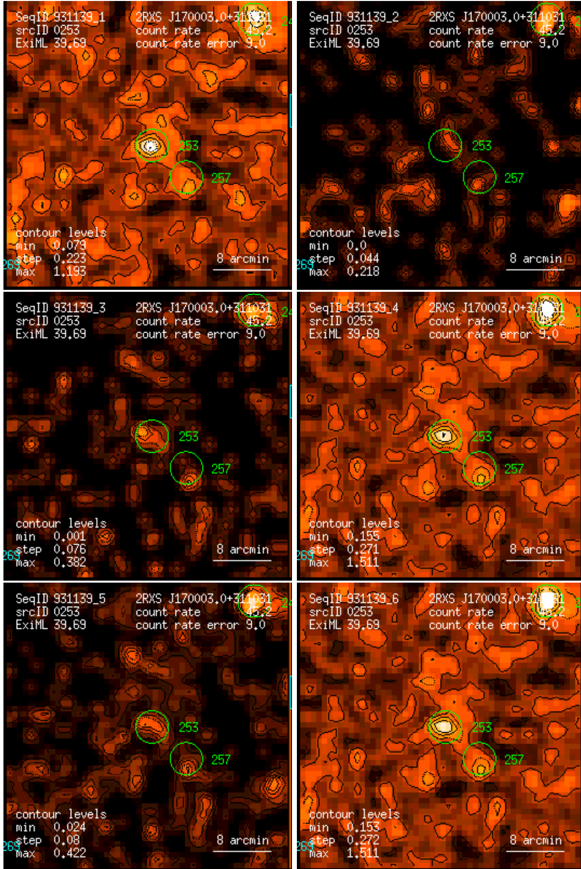
Figure 253: RASS 931139: detection 0253: band rate images, Gaussian filter: (1) PSPC channels 11 – 41, (2) 52 – 90, (3) 91 – 201, (4) 11 – 235, (5) 52 – 201, (6) 11 – 201. Broad band rates in counts/ks. Band rate contour levels in counts/ks/arcmin 2 .
