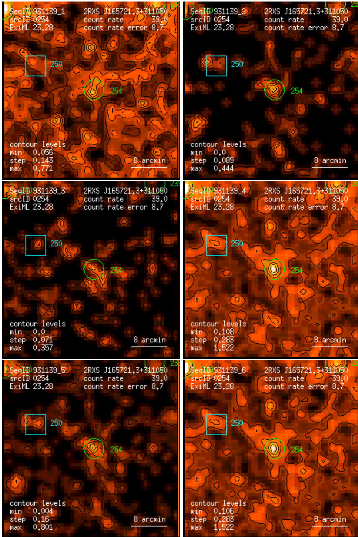
Figure 254: RASS 931139: detection 0254: band rate images, Gaussian filter: (1) PSPC channels 11 – 41, (2) 52 – 90, (3) 91 – 201, (4) 11 – 235, (5) 52 – 201, (6) 11 – 201. Broad band rates in counts/ks. Band rate contour levels in counts/ks/arcmin 2 .
