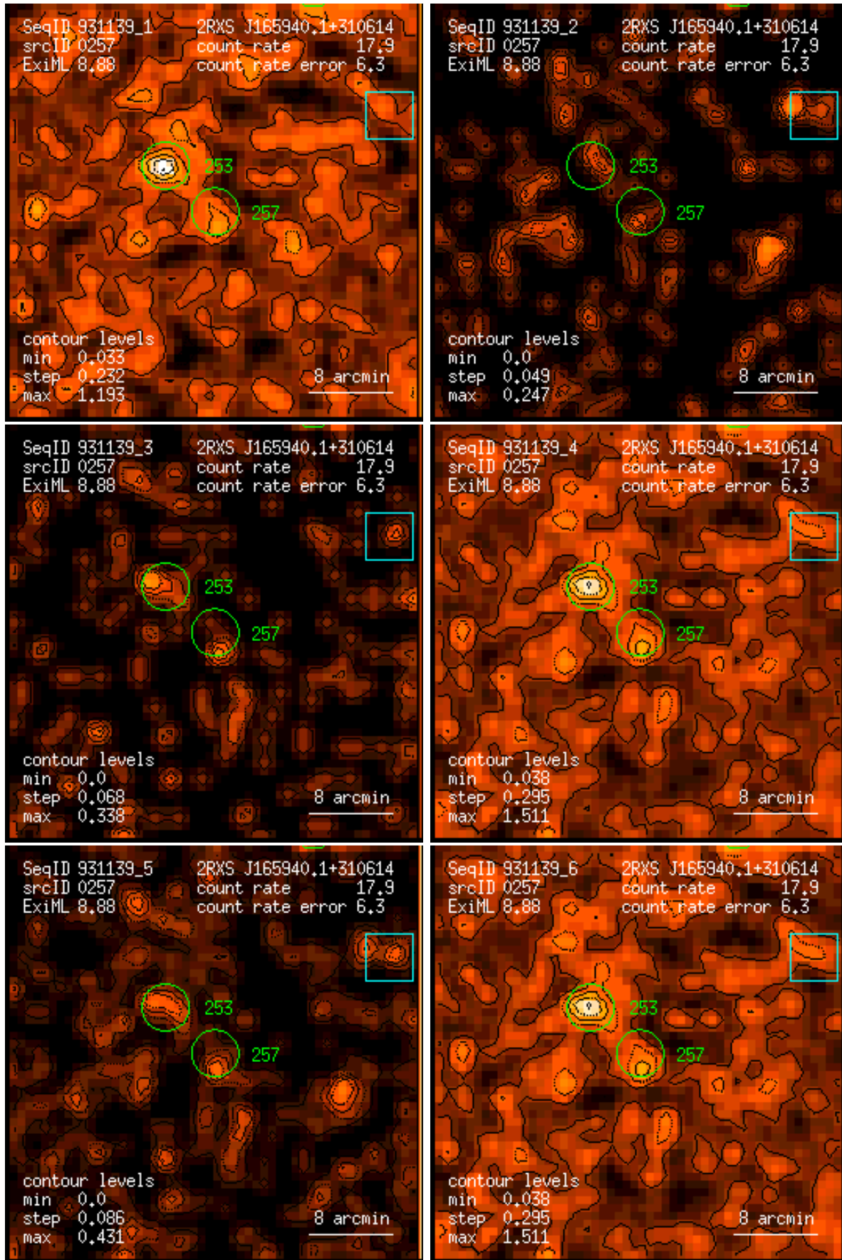
Figure 257: RASS 931139: detection 0257: band rate images, Gaussian filter: (1) PSPC channels 11 – 41, (2) 52 – 90, (3) 91 – 201, (4) 11 – 235, (5) 52 – 201, (6) 11 – 201. Broad band rates in counts/ks. Band rate contour levels in counts/ks/arcmin 2 .
