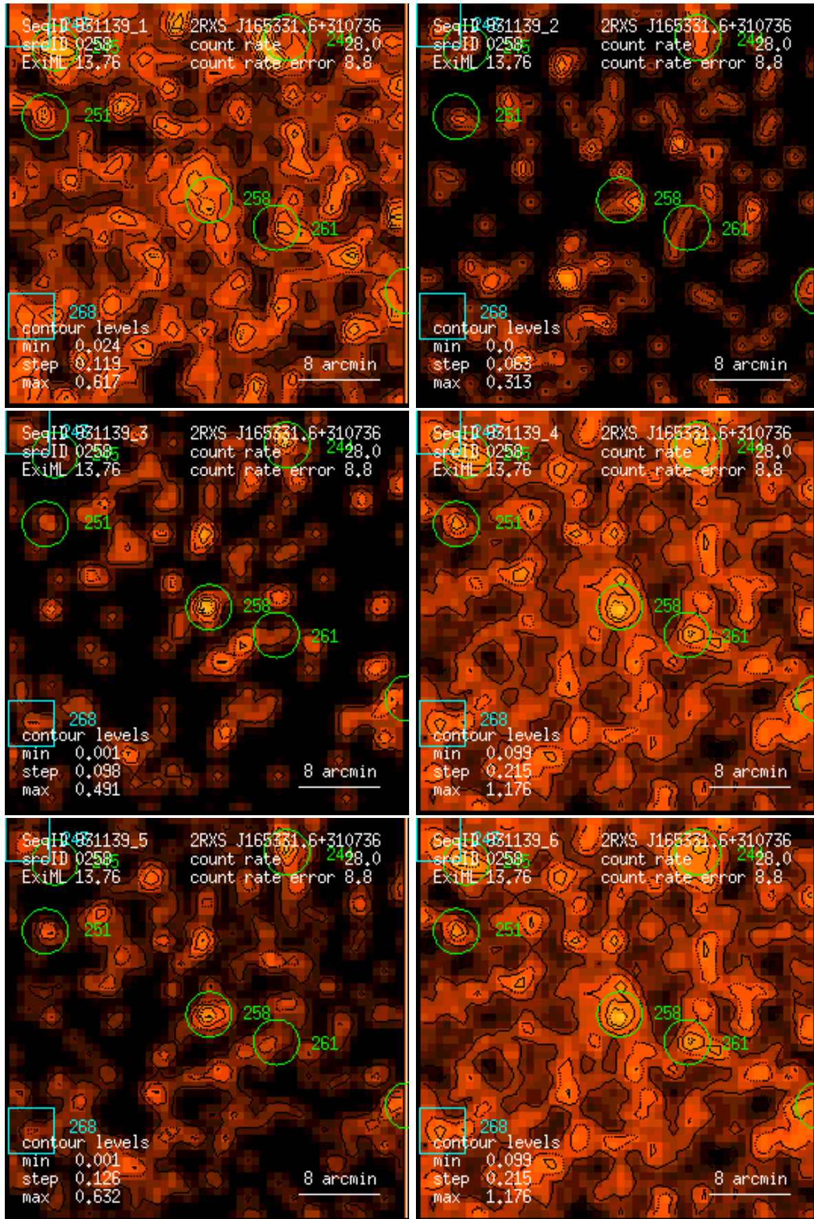
Figure 258: RASS 931139: detection 0258: band rate images, Gaussian filter: (1) PSPC channels 11 – 41, (2) 52 – 90, (3) 91 – 201, (4) 11 – 235, (5) 52 – 201, (6) 11 – 201. Broad band rates in counts/ks. Band rate contour levels in counts/ks/arcmin 2 .
