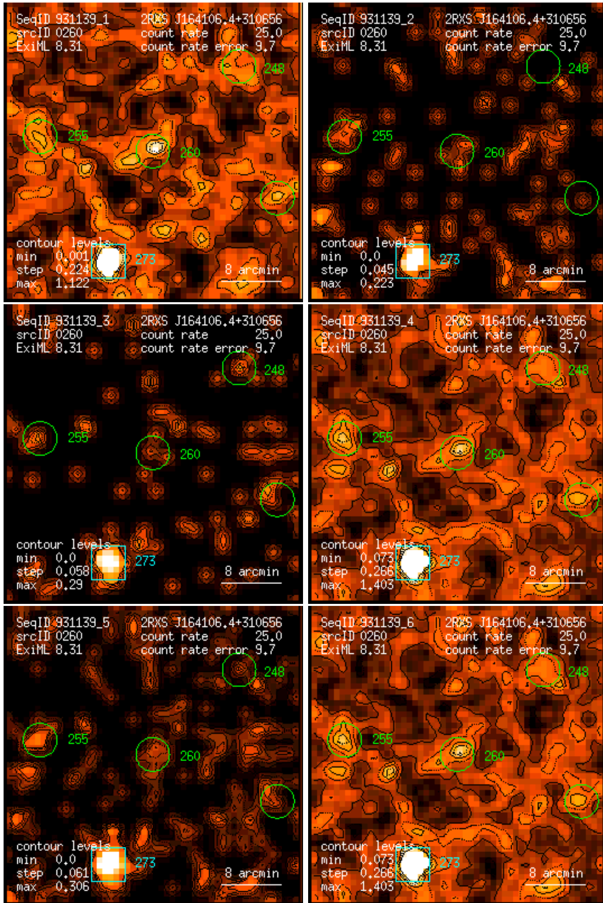
Figure 260: RASS 931139: detection 0260: band rate images, Gaussian filter: (1) PSPC channels 11 – 41, (2) 52 – 90, (3) 91 – 201, (4) 11 – 235, (5) 52 – 201, (6) 11 – 201. Broad band rates in counts/ks. Band rate contour levels in counts/ks/arcmin 2 .
