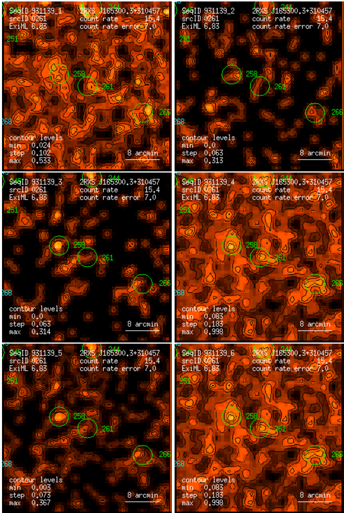
Figure 261: RASS 931139: detection 0261: band rate images, Gaussian filter: (1) PSPC channels 11 – 41, (2) 52 – 90, (3) 91 – 201, (4) 11 – 235, (5) 52 – 201, (6) 11 – 201. Broad band rates in counts/ks. Band rate contour levels in counts/ks/arcmin 2 .
