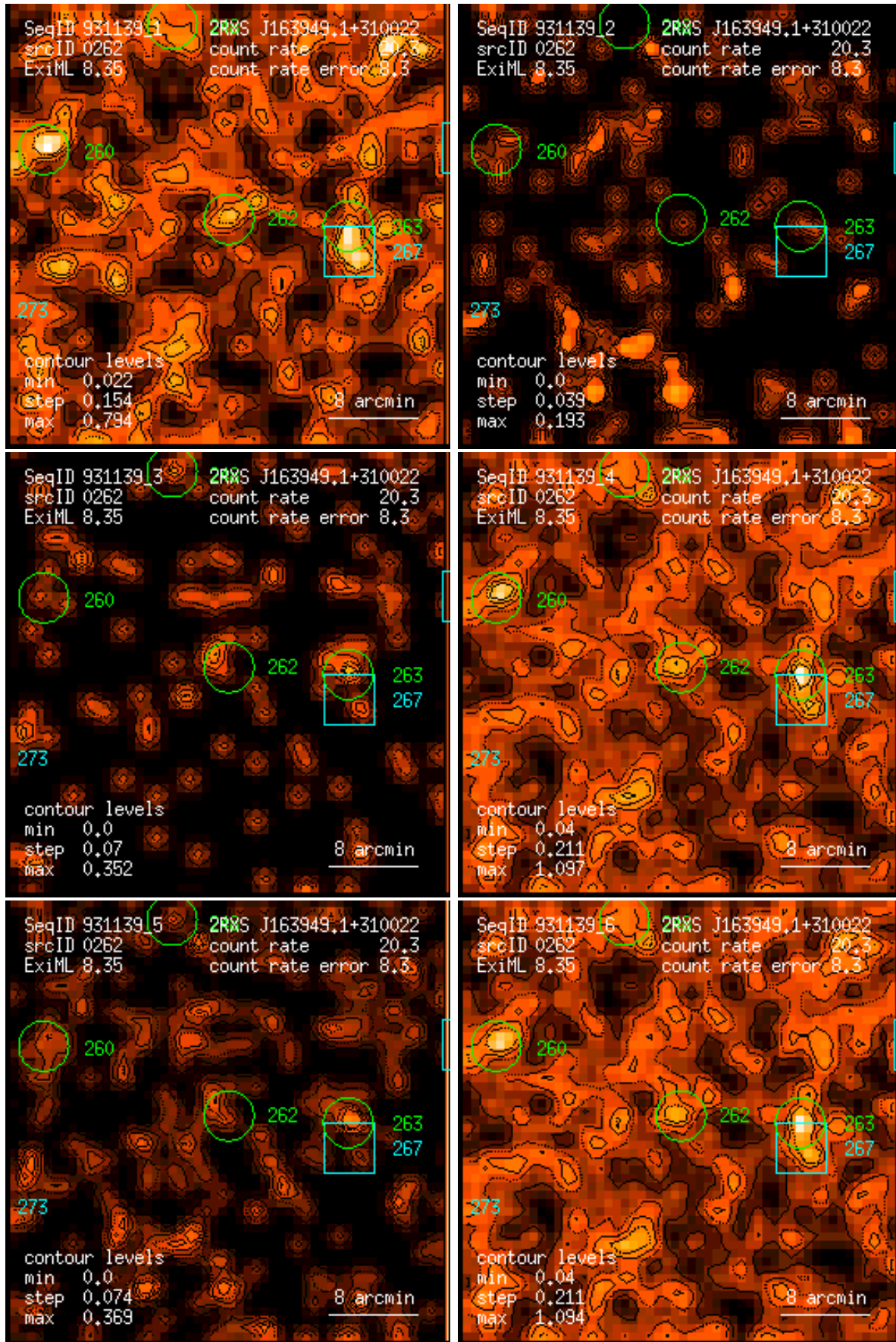
Figure 262: RASS 931139: detection 0262: band rate images, Gaussian filter: (1) PSPC channels 11 – 41, (2) 52 – 90, (3) 91 – 201, (4) 11 – 235, (5) 52 – 201, (6) 11 – 201. Broad band rates in counts/ks. Band rate contour levels in counts/ks/arcmin 2 .
