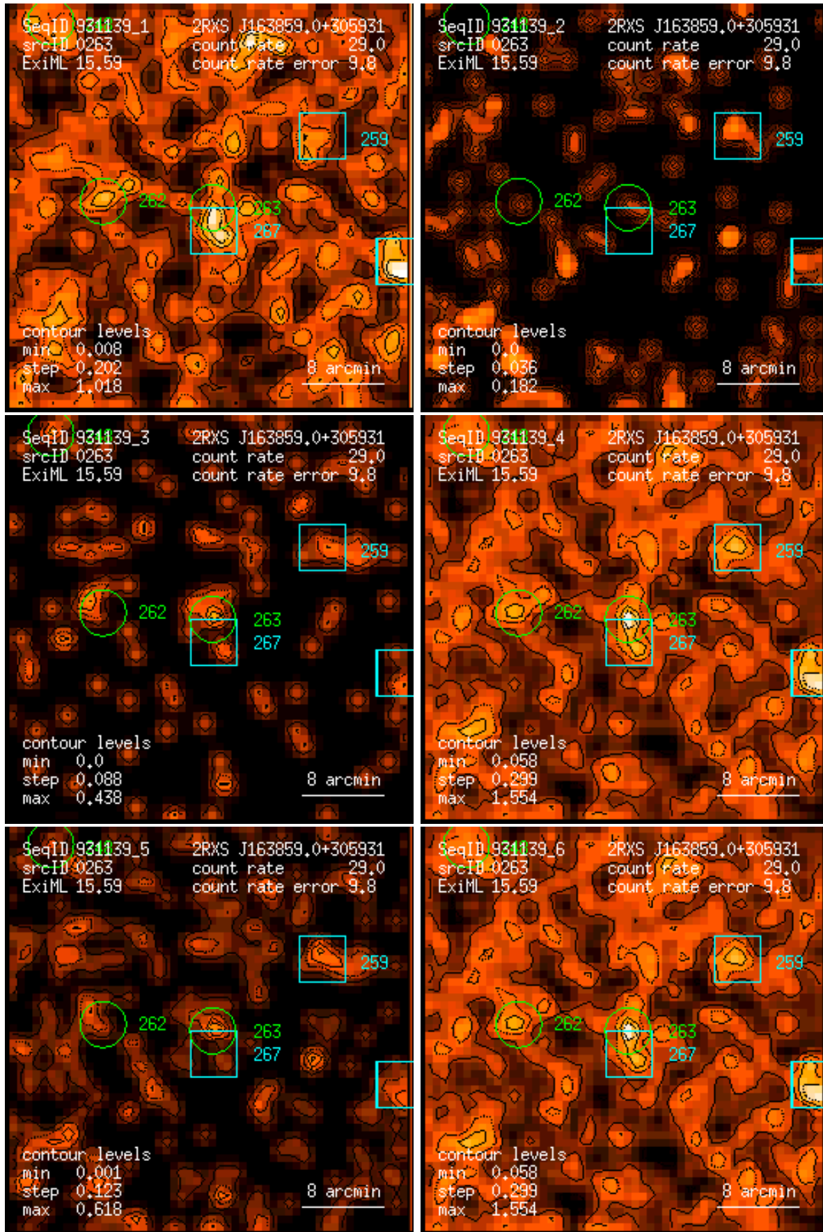
Figure 263: RASS 931139: detection 0263: band rate images, Gaussian filter: (1) PSPC channels 11 – 41, (2) 52 – 90, (3) 91 – 201, (4) 11 – 235, (5) 52 – 201, (6) 11 – 201. Broad band rates in counts/ks. Band rate contour levels in counts/ks/arcmin 2 .
