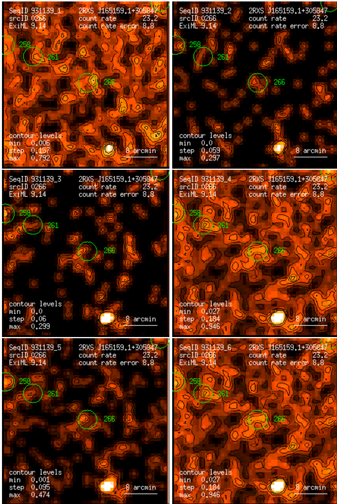
Figure 266: RASS 931139: detection 0266: band rate images, Gaussian filter: (1) PSPC channels 11 – 41, (2) 52 – 90, (3) 91 – 201, (4) 11 – 235, (5) 52 – 201, (6) 11 – 201. Broad band rates in counts/ks. Band rate contour levels in counts/ks/arcmin 2 .
