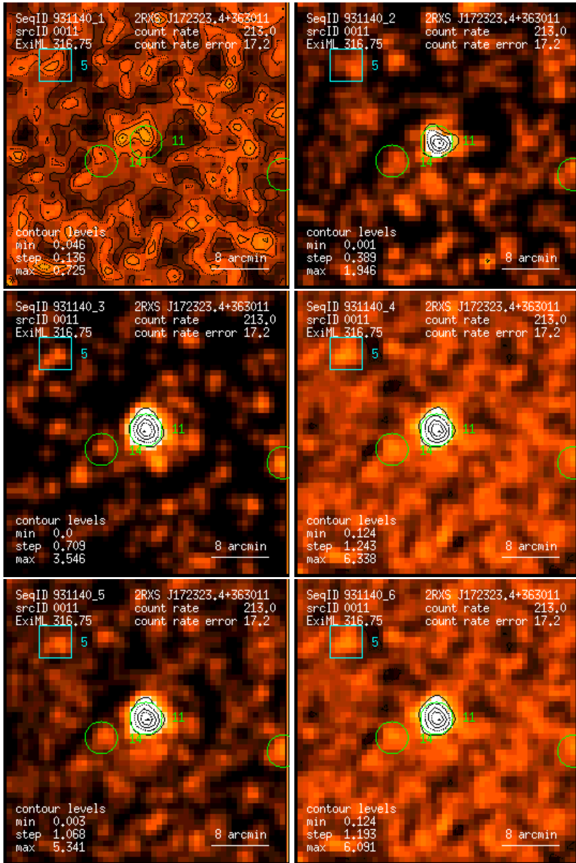
Figure 11: RASS 931140: detection 0011: band rate images, Gaussian filter: (1) PSPC channels 11 – 41, (2) 52 – 90, (3) 91 – 201, (4) 11 – 235, (5) 52 – 201, (6) 11 – 201. Broad band rates in counts/ks. Band rate contour levels in counts/ks/arcmin 2 .
