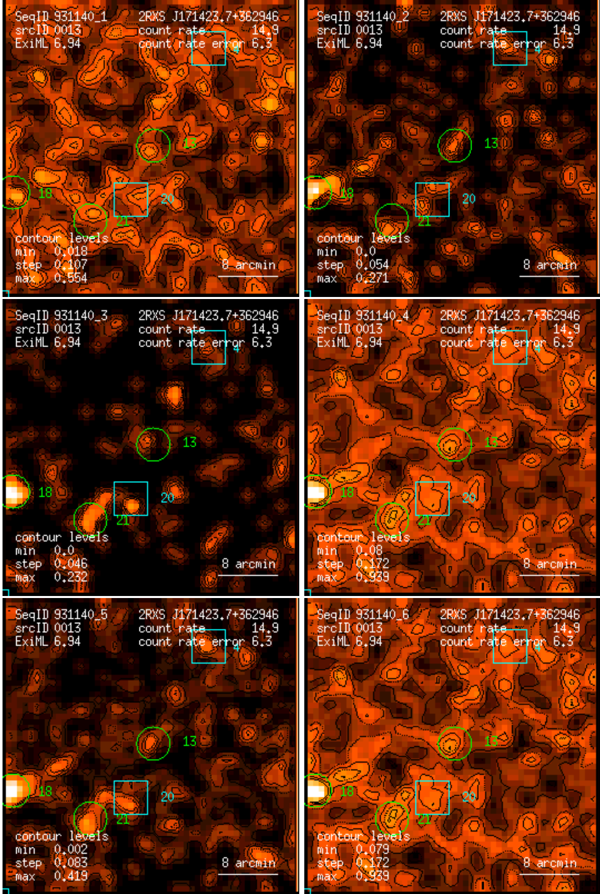
Figure 13: RASS 931140: detection 0013: band rate images, Gaussian filter: (1) PSPC channels 11 – 41, (2) 52 – 90, (3) 91 – 201, (4) 11 – 235, (5) 52 – 201, (6) 11 – 201. Broad band rates in counts/ks. Band rate contour levels in counts/ks/arcmin 2 .
