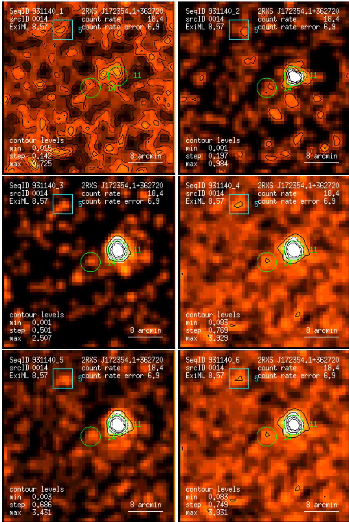
Figure 14: RASS 931140: detection 0014: band rate images, Gaussian filter: (1) PSPC channels 11 – 41, (2) 52 – 90, (3) 91 – 201, (4) 11 – 235, (5) 52 – 201, (6) 11 – 201. Broad band rates in counts/ks. Band rate contour levels in counts/ks/arcmin 2 .
