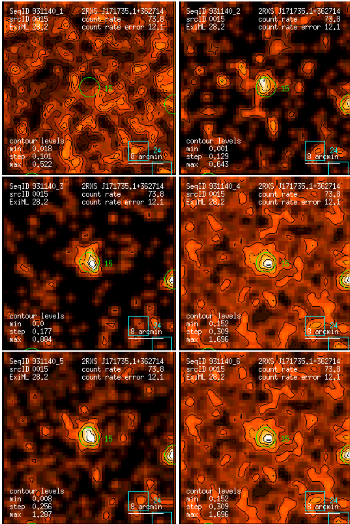
Figure 15: RASS 931140: detection 0015: band rate images, Gaussian filter: (1) PSPC channels 11 – 41, (2) 52 – 90, (3) 91 – 201, (4) 11 – 235, (5) 52 – 201, (6) 11 – 201. Broad band rates in counts/ks. Band rate contour levels in counts/ks/arcmin 2 .
