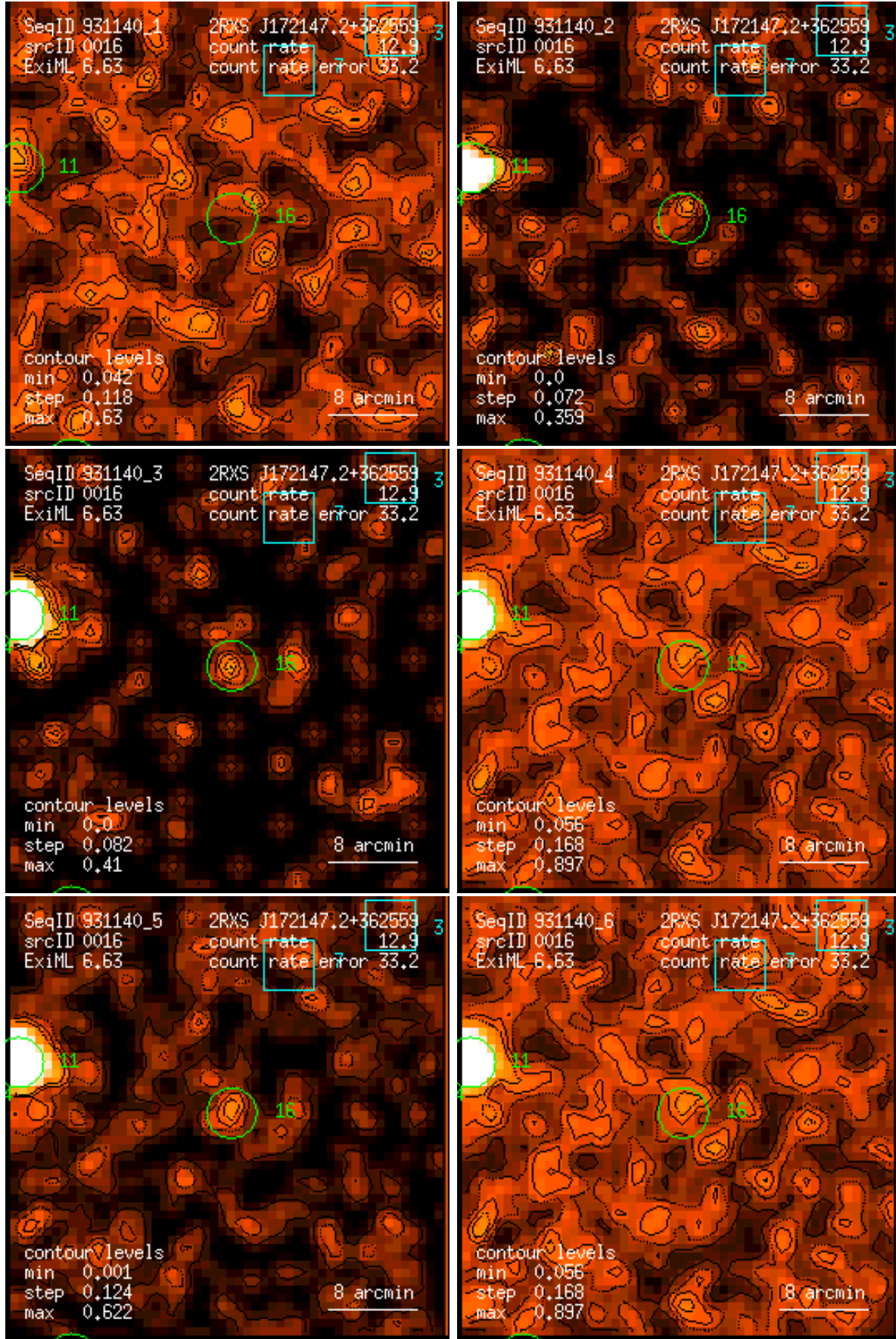
Figure 16: RASS 931140: detection 0016: band rate images, Gaussian filter: (1) PSPC channels 11 – 41, (2) 52 – 90, (3) 91 – 201, (4) 11 – 235, (5) 52 – 201, (6) 11 – 201. Broad band rates in counts/ks. Band rate contour levels in counts/ks/arcmin 2 .
