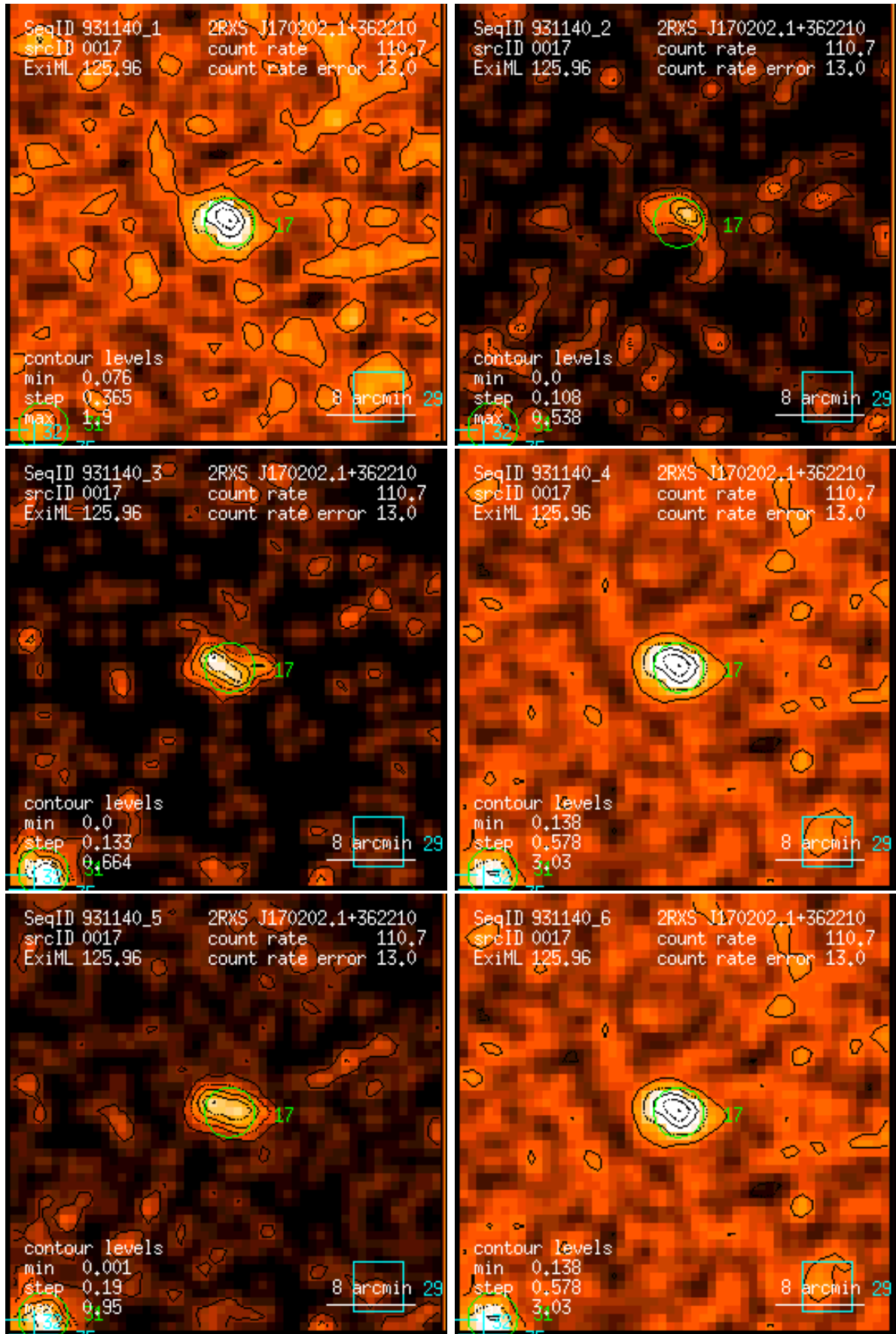
Figure 17: RASS 931140: detection 0017: band rate images, Gaussian filter: (1) PSPC channels 11 – 41, (2) 52 – 90, (3) 91 – 201, (4) 11 – 235, (5) 52 – 201, (6) 11 – 201. Broad band rates in counts/ks. Band rate contour levels in counts/ks/arcmin 2 .
