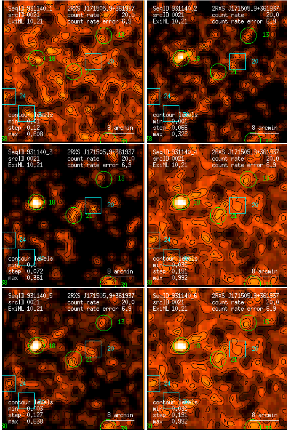
Figure 21: RASS 931140: detection 0021: band rate images, Gaussian filter: (1) PSPC channels 11 – 41, (2) 52 – 90, (3) 91 – 201, (4) 11 – 235, (5) 52 – 201, (6) 11 – 201. Broad band rates in counts/ks. Band rate contour levels in counts/ks/arcmin 2 .
