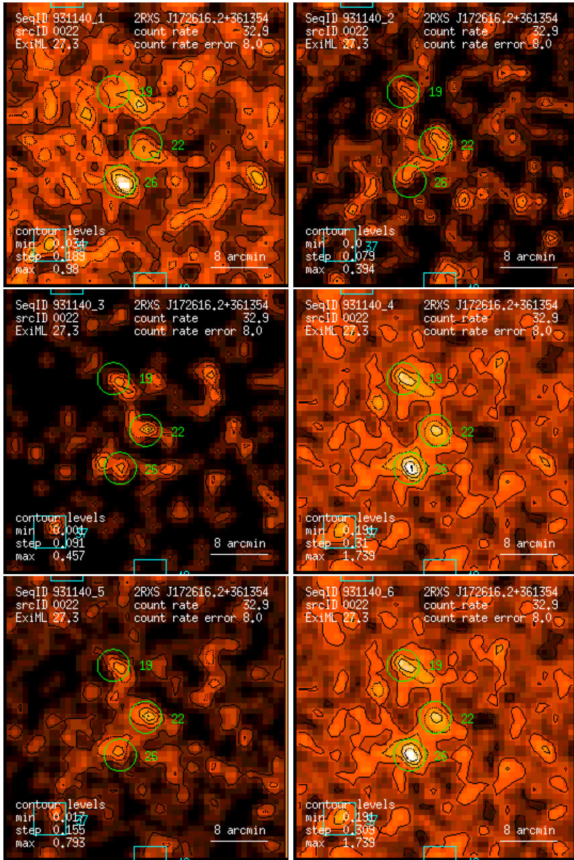
Figure 22: RASS 931140: detection 0022: band rate images, Gaussian filter: (1) PSPC channels 11 – 41, (2) 52 – 90, (3) 91 – 201, (4) 11 – 235, (5) 52 – 201, (6) 11 – 201. Broad band rates in counts/ks. Band rate contour levels in counts/ks/arcmin 2 .
