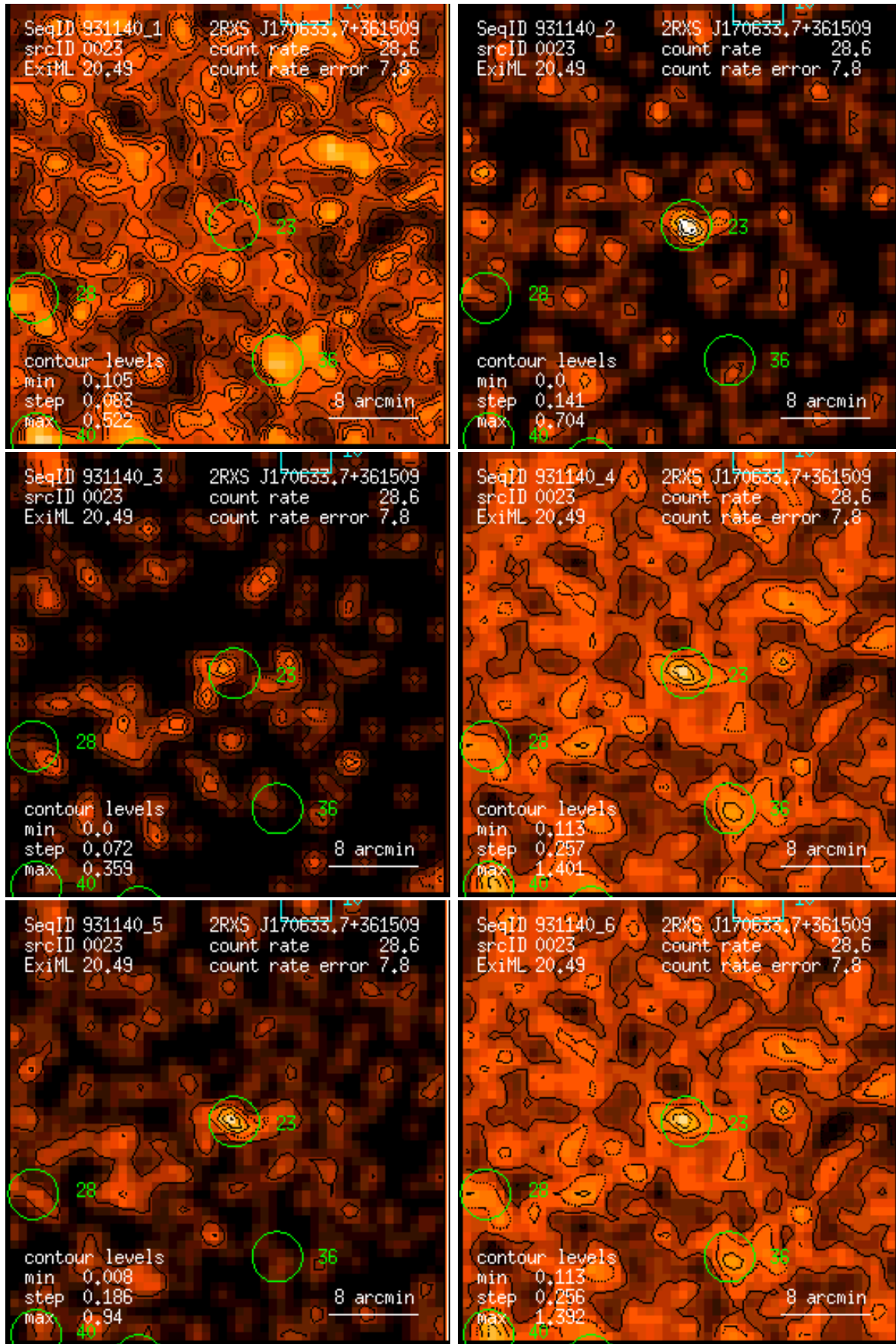
Figure 23: RASS 931140: detection 0023: band rate images, Gaussian filter: (1) PSPC channels 11 – 41, (2) 52 – 90, (3) 91 – 201, (4) 11 – 235, (5) 52 – 201, (6) 11 – 201. Broad band rates in counts/ks. Band rate contour levels in counts/ks/arcmin 2 .
