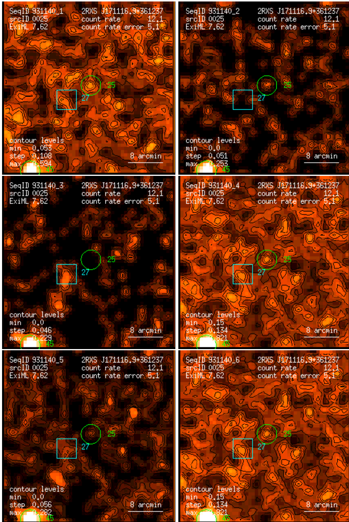
Figure 25: RASS 931140: detection 0025: band rate images, Gaussian filter: (1) PSPC channels 11 – 41, (2) 52 – 90, (3) 91 – 201, (4) 11 – 235, (5) 52 – 201, (6) 11 – 201. Broad band rates in counts/ks. Band rate contour levels in counts/ks/arcmin 2 .
