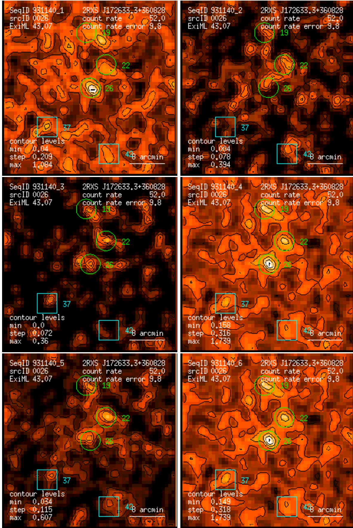
Figure 26: RASS 931140: detection 0026: band rate images, Gaussian filter: (1) PSPC channels 11 – 41, (2) 52 – 90, (3) 91 – 201, (4) 11 – 235, (5) 52 – 201, (6) 11 – 201. Broad band rates in counts/ks. Band rate contour levels in counts/ks/arcmin 2 .
