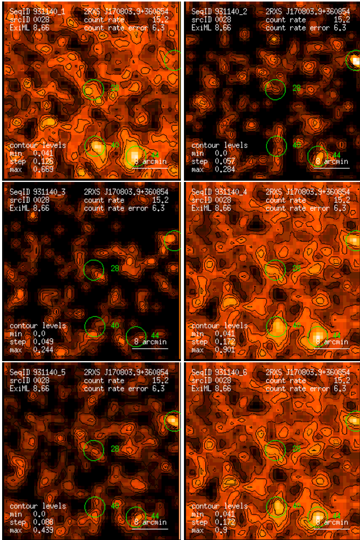
Figure 28: RASS 931140: detection 0028: band rate images, Gaussian filter: (1) PSPC channels 11 – 41, (2) 52 – 90, (3) 91 – 201, (4) 11 – 235, (5) 52 – 201, (6) 11 – 201. Broad band rates in counts/ks. Band rate contour levels in counts/ks/arcmin 2 .
