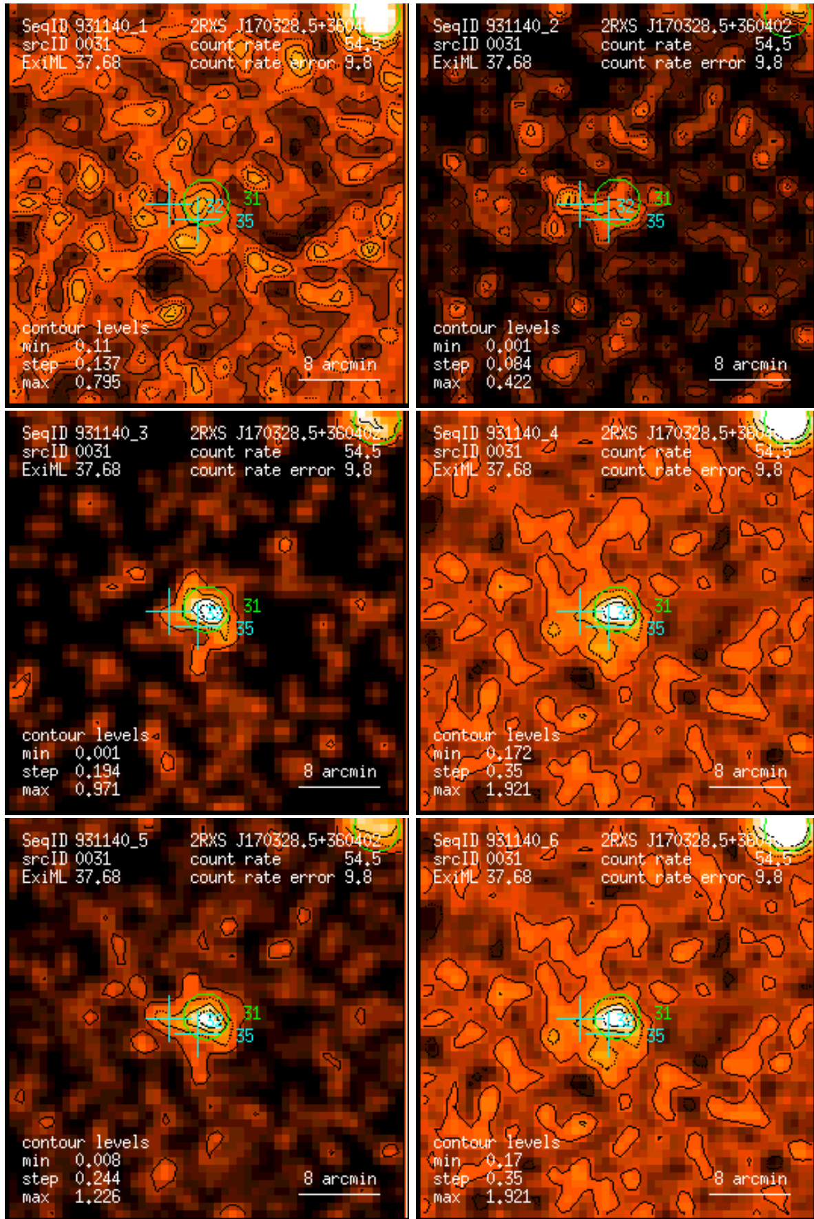
Figure 31: RASS 931140: detection 0031: band rate images, Gaussian filter: (1) PSPC channels 11 – 41, (2) 52 – 90, (3) 91 – 201, (4) 11 – 235, (5) 52 – 201, (6) 11 – 201. Broad band rates in counts/ks. Band rate contour levels in counts/ks/arcmin 2 .
