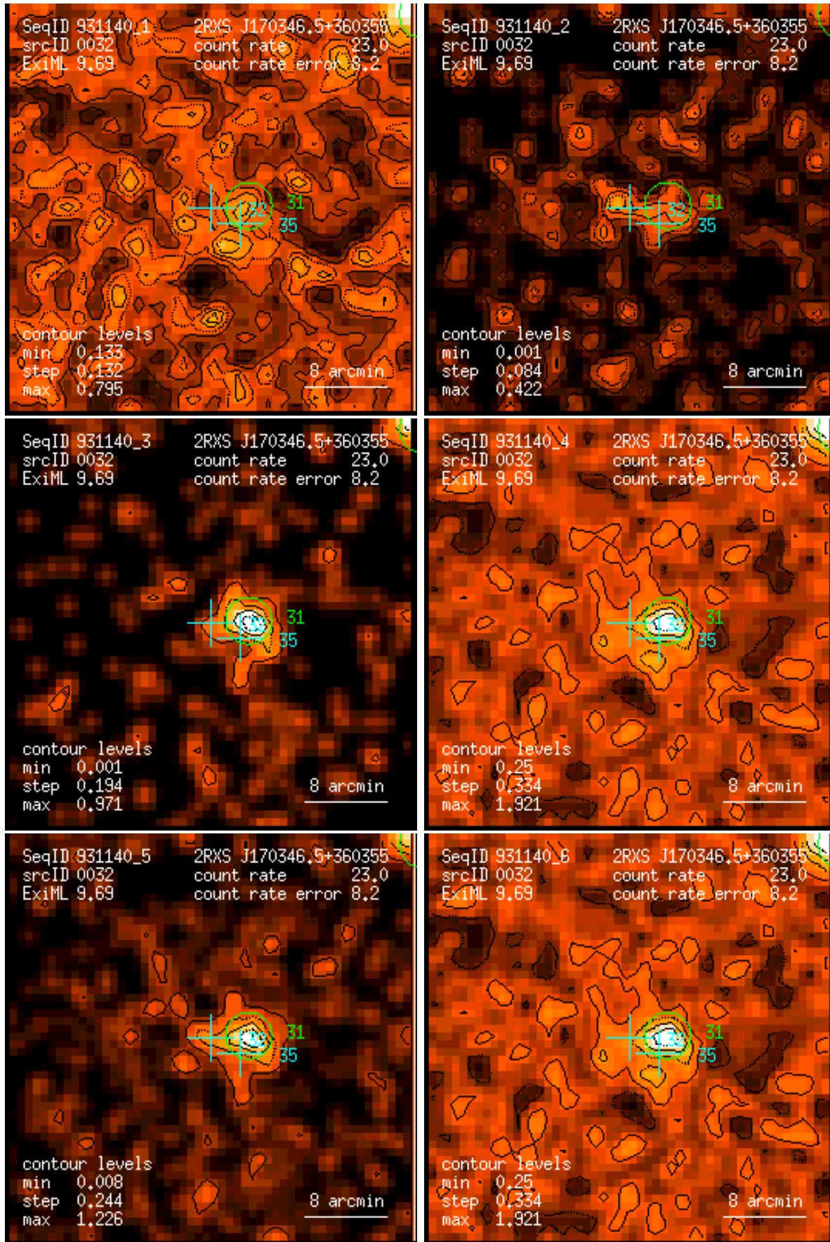
Figure 32: RASS 931140: detection 0032: band rate images, Gaussian filter: (1) PSPC channels 11 – 41, (2) 52 – 90, (3) 91 – 201, (4) 11 – 235, (5) 52 – 201, (6) 11 – 201. Broad band rates in counts/ks. Band rate contour levels in counts/ks/arcmin 2 .
