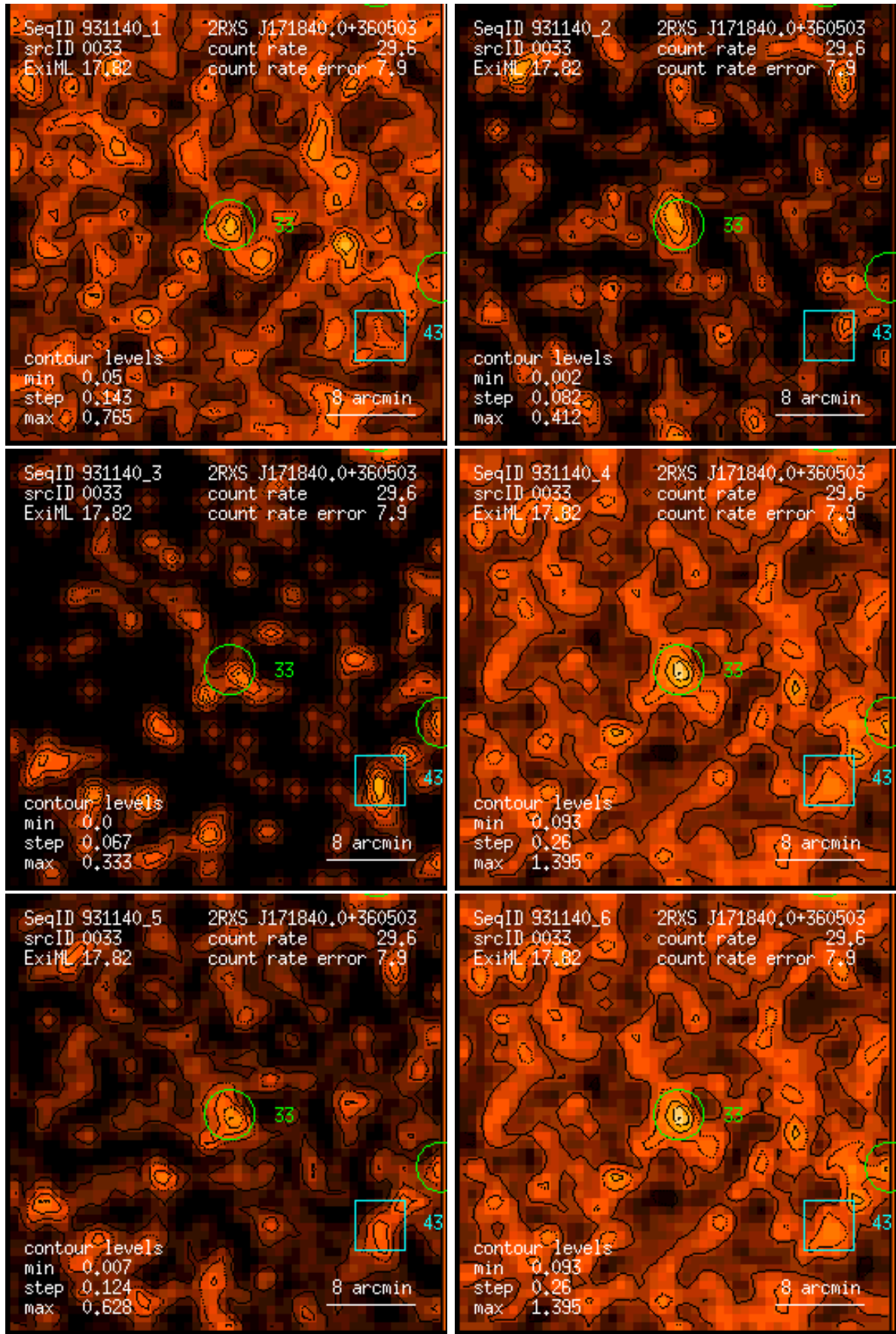
Figure 33: RASS 931140: detection 0033: band rate images, Gaussian filter: (1) PSPC channels 11 – 41, (2) 52 – 90, (3) 91 – 201, (4) 11 – 235, (5) 52 – 201, (6) 11 – 201. Broad band rates in counts/ks. Band rate contour levels in counts/ks/arcmin 2 .
