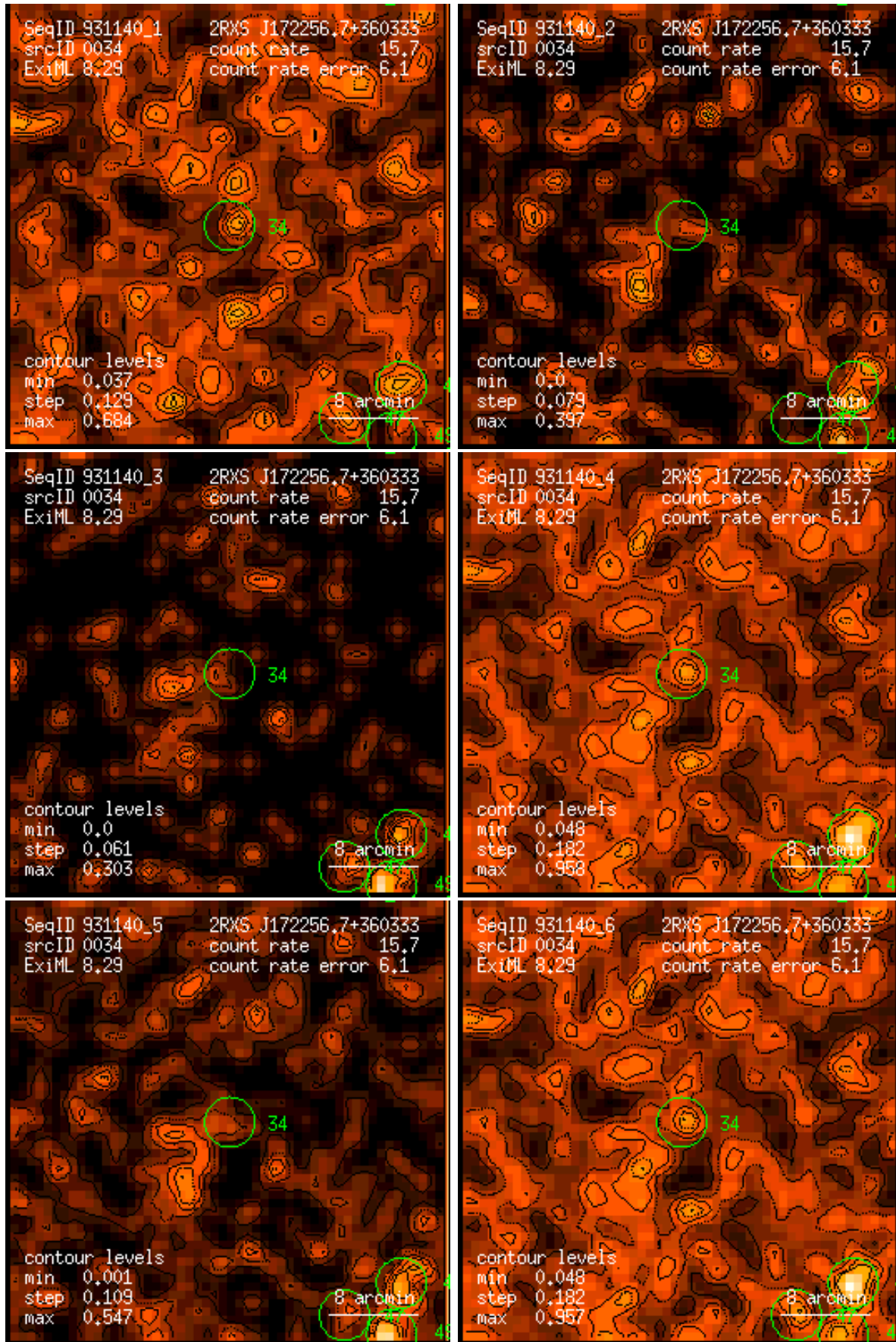
Figure 34: RASS 931140: detection 0034: band rate images, Gaussian filter: (1) PSPC channels 11 – 41, (2) 52 – 90, (3) 91 – 201, (4) 11 – 235, (5) 52 – 201, (6) 11 – 201. Broad band rates in counts/ks. Band rate contour levels in counts/ks/arcmin 2 .
