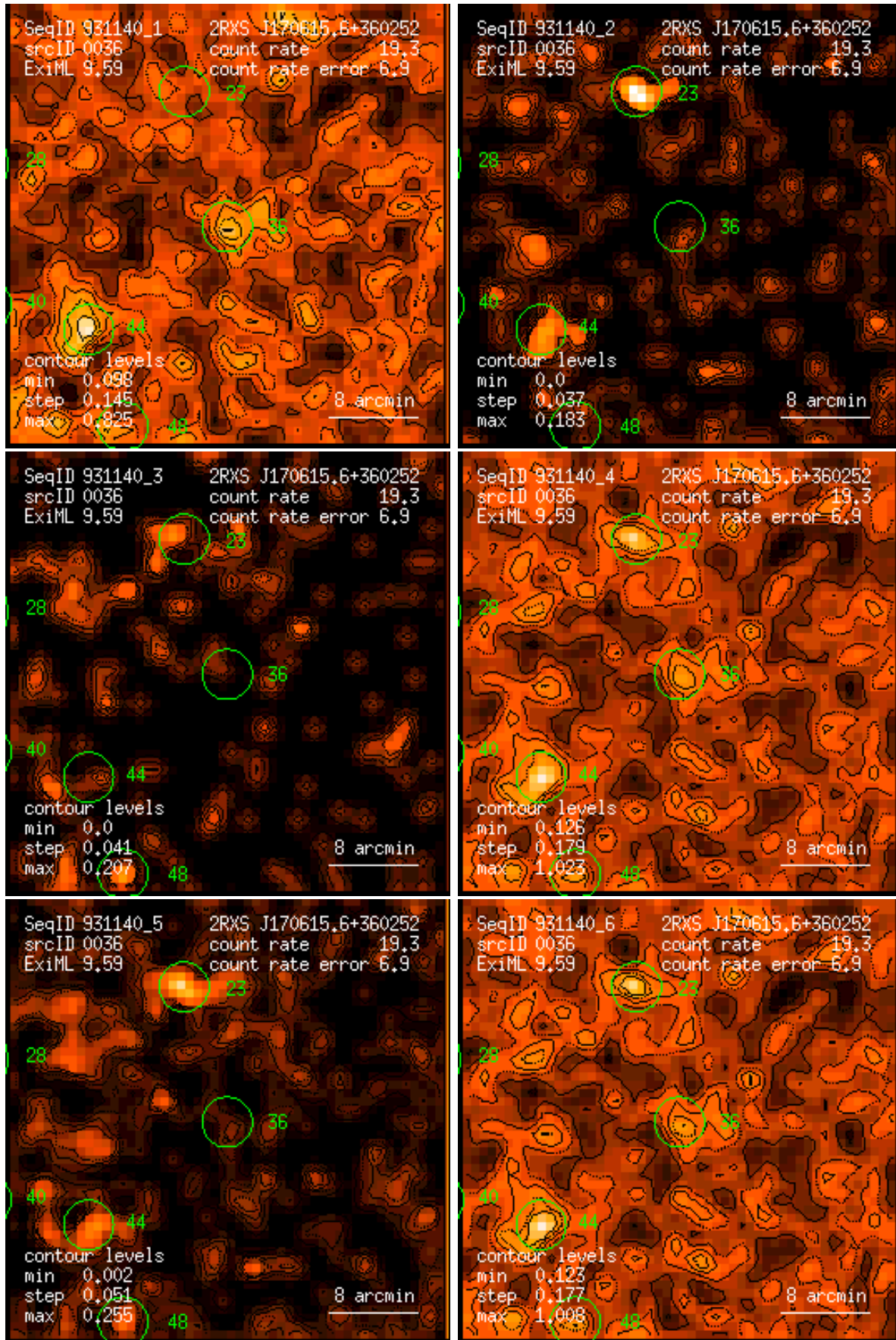
Figure 36: RASS 931140: detection 0036: band rate images, Gaussian filter: (1) PSPC channels 11 – 41, (2) 52 – 90, (3) 91 – 201, (4) 11 – 235, (5) 52 – 201, (6) 11 – 201. Broad band rates in counts/ks. Band rate contour levels in counts/ks/arcmin 2 .
