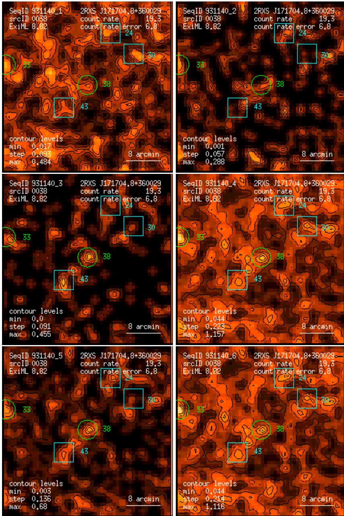
Figure 38: RASS 931140: detection 0038: band rate images, Gaussian filter: (1) PSPC channels 11 – 41, (2) 52 – 90, (3) 91 – 201, (4) 11 – 235, (5) 52 – 201, (6) 11 – 201. Broad band rates in counts/ks. Band rate contour levels in counts/ks/arcmin 2 .
