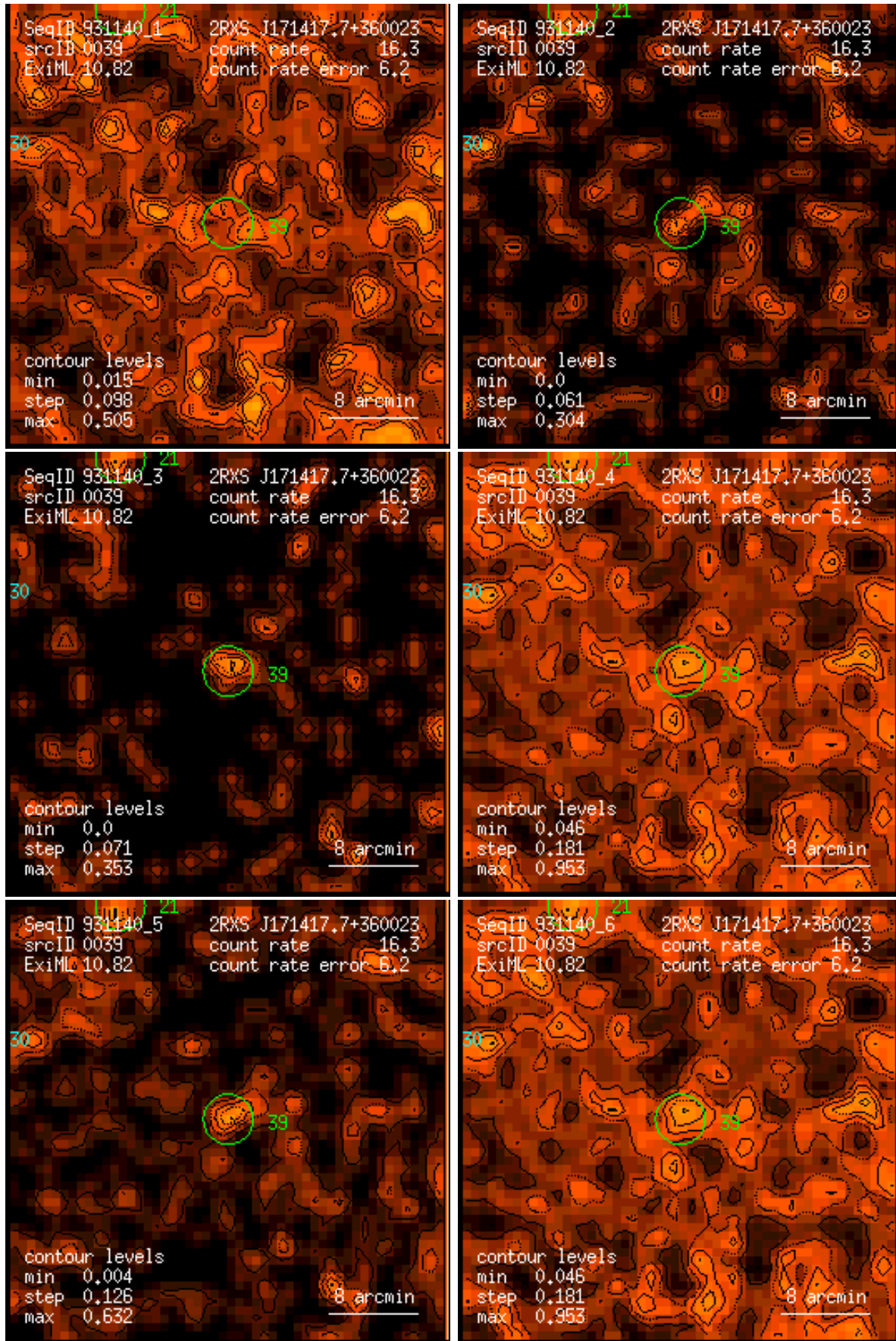
Figure 39: RASS 931140: detection 0039: band rate images, Gaussian filter: (1) PSPC channels 11 – 41, (2) 52 – 90, (3) 91 – 201, (4) 11 – 235, (5) 52 – 201, (6) 11 – 201. Broad band rates in counts/ks. Band rate contour levels in counts/ks/arcmin 2 .
