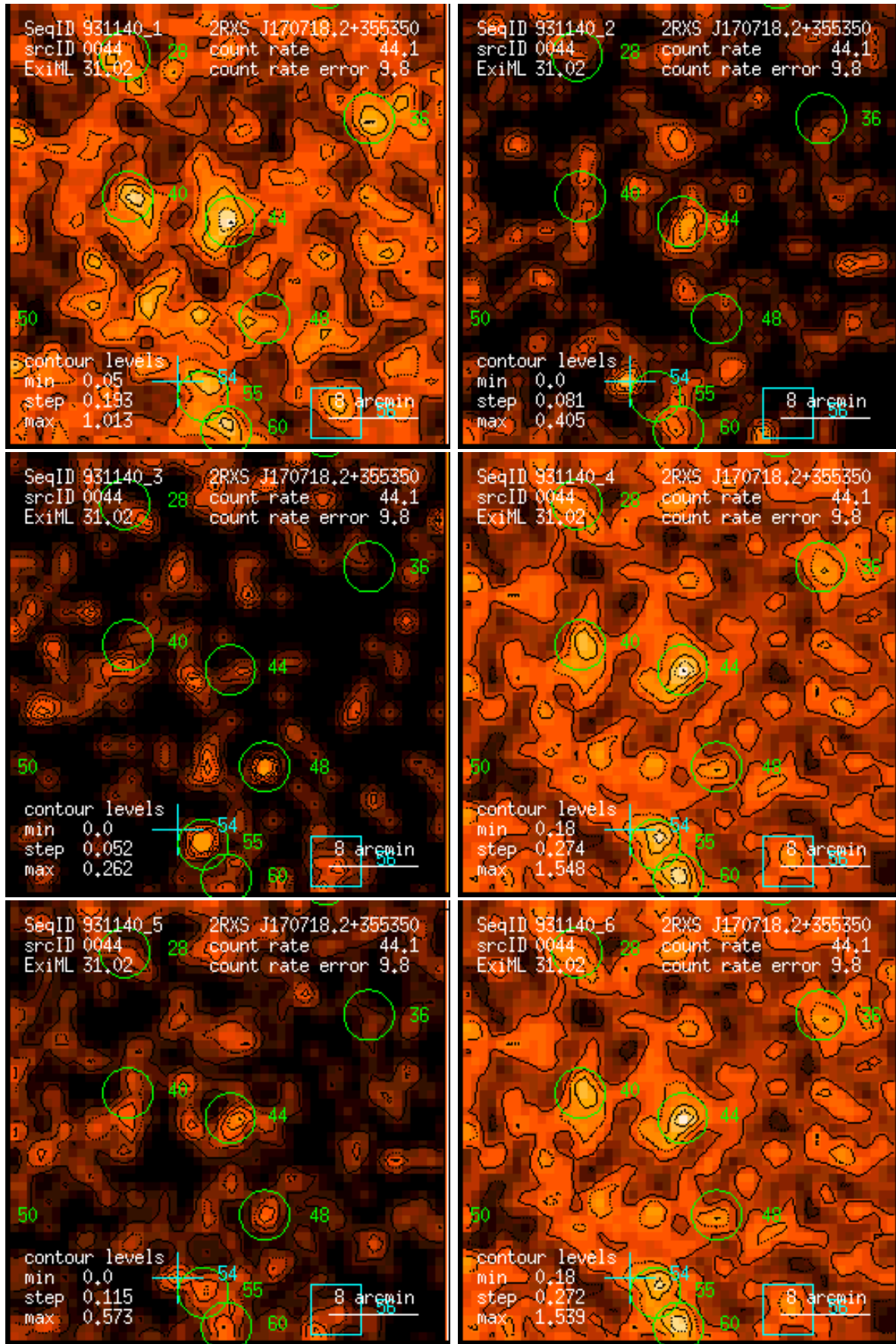
Figure 44: RASS 931140: detection 0044: band rate images, Gaussian filter: (1) PSPC channels 11 – 41, (2) 52 – 90, (3) 91 – 201, (4) 11 – 235, (5) 52 – 201, (6) 11 – 201. Broad band rates in counts/ks. Band rate contour levels in counts/ks/arcmin 2 .
