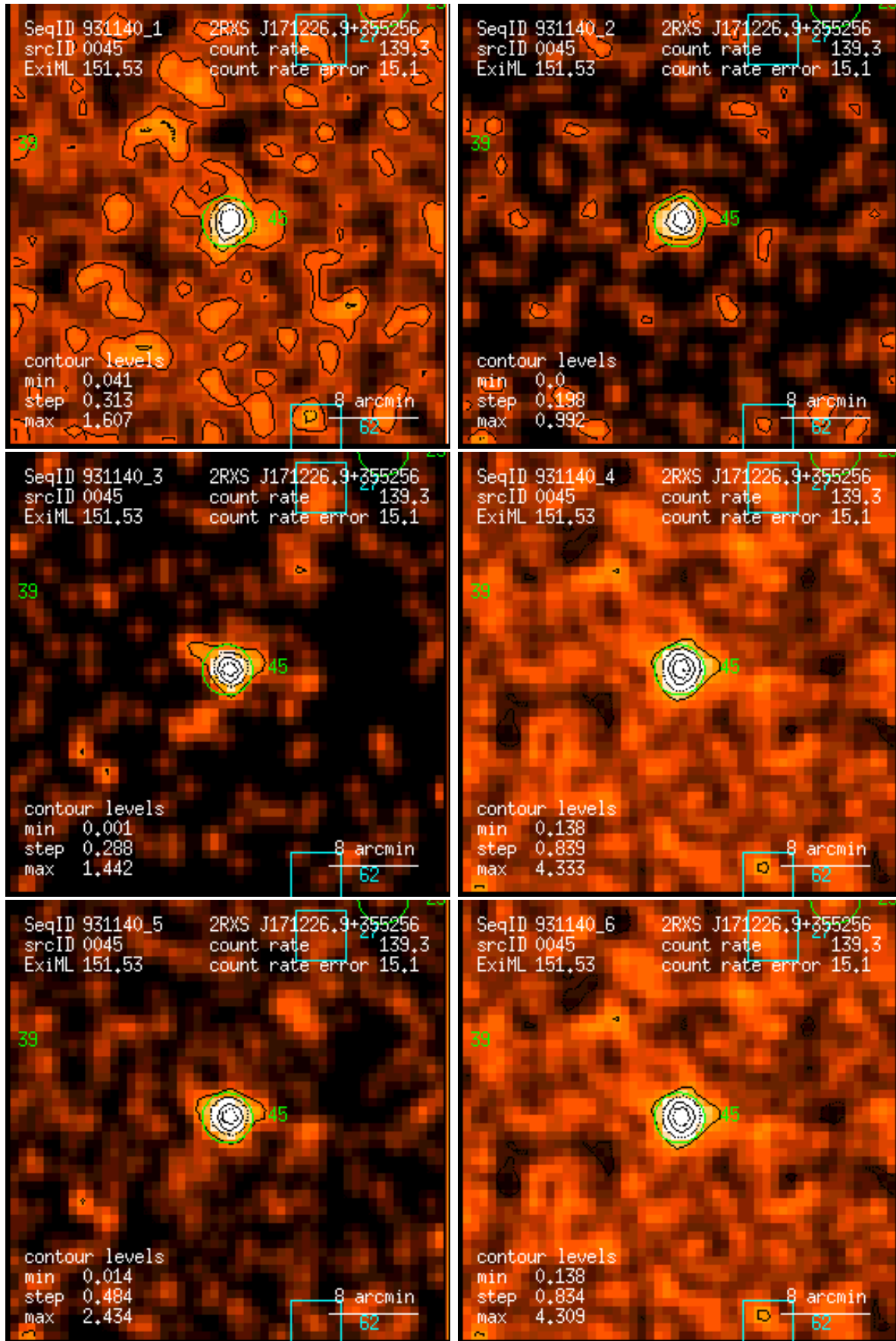
Figure 45: RASS 931140: detection 0045: band rate images, Gaussian filter: (1) PSPC channels 11 – 41, (2) 52 – 90, (3) 91 – 201, (4) 11 – 235, (5) 52 – 201, (6) 11 – 201. Broad band rates in counts/ks. Band rate contour levels in counts/ks/arcmin 2 .
