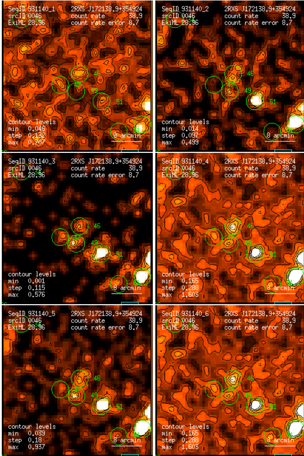
Figure 46: RASS 931140: detection 0046: band rate images, Gaussian filter: (1) PSPC channels 11 – 41, (2) 52 – 90, (3) 91 – 201, (4) 11 – 235, (5) 52 – 201, (6) 11 – 201. Broad band rates in counts/ks. Band rate contour levels in counts/ks/arcmin 2 .
