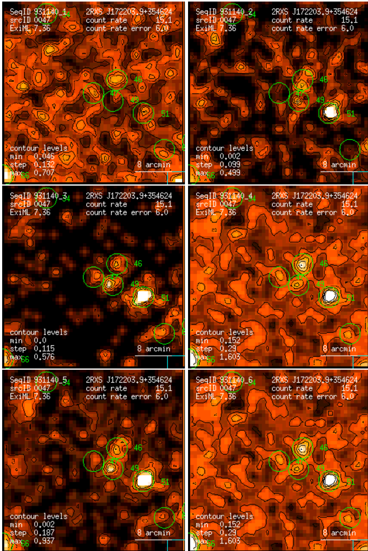
Figure 47: RASS 931140: detection 0047: band rate images, Gaussian filter: (1) PSPC channels 11 – 41, (2) 52 – 90, (3) 91 – 201, (4) 11 – 235, (5) 52 – 201, (6) 11 – 201. Broad band rates in counts/ks. Band rate contour levels in counts/ks/arcmin 2 .
