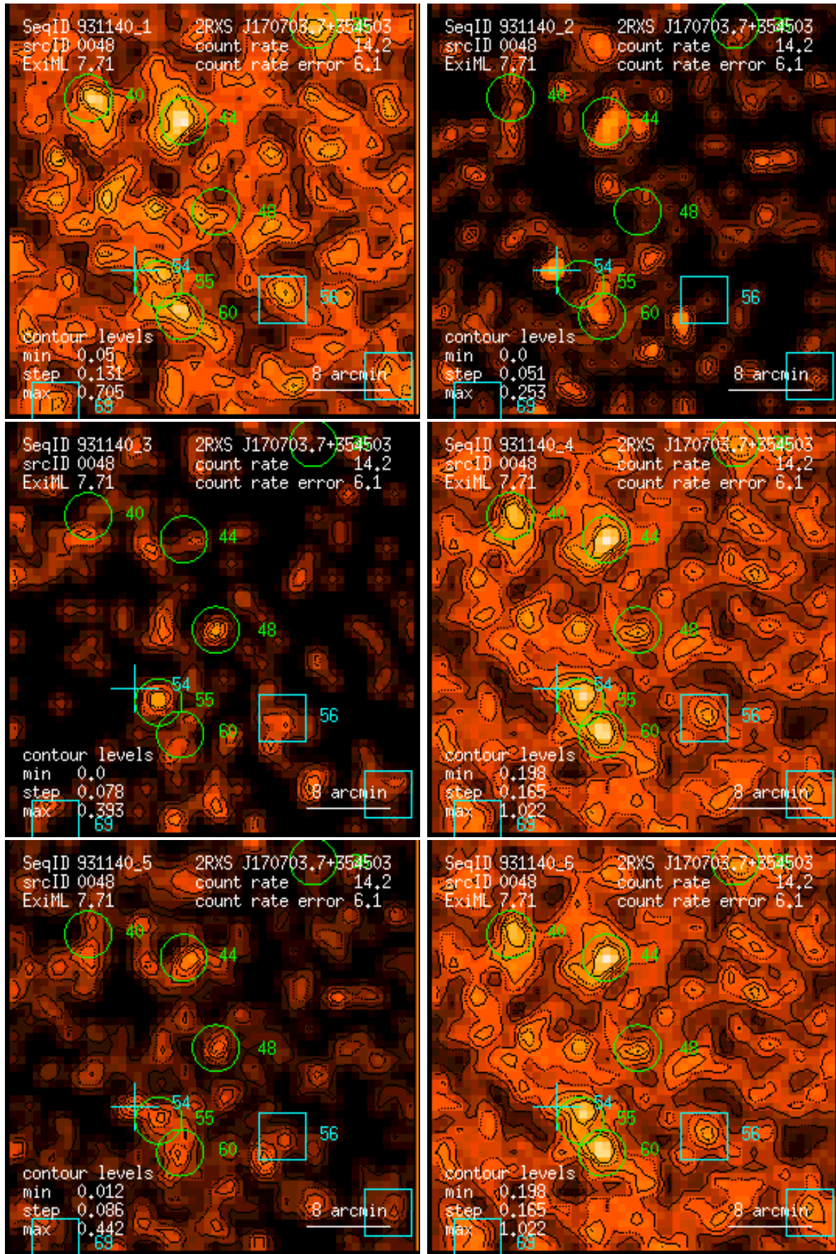
Figure 48: RASS 931140: detection 0048: band rate images, Gaussian filter: (1) PSPC channels 11 – 41, (2) 52 – 90, (3) 91 – 201, (4) 11 – 235, (5) 52 – 201, (6) 11 – 201. Broad band rates in counts/ks. Band rate contour levels in counts/ks/arcmin 2 .
