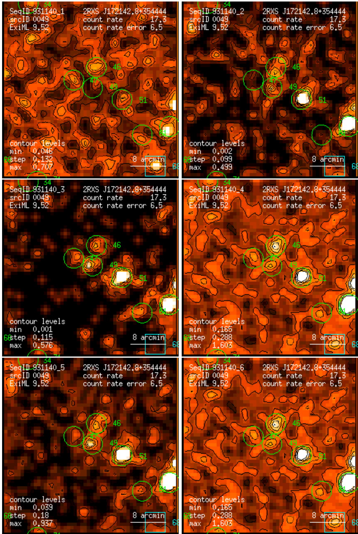
Figure 49: RASS 931140: detection 0049: band rate images, Gaussian filter: (1) PSPC channels 11 – 41, (2) 52 – 90, (3) 91 – 201, (4) 11 – 235, (5) 52 – 201, (6) 11 – 201. Broad band rates in counts/ks. Band rate contour levels in counts/ks/arcmin 2 .
