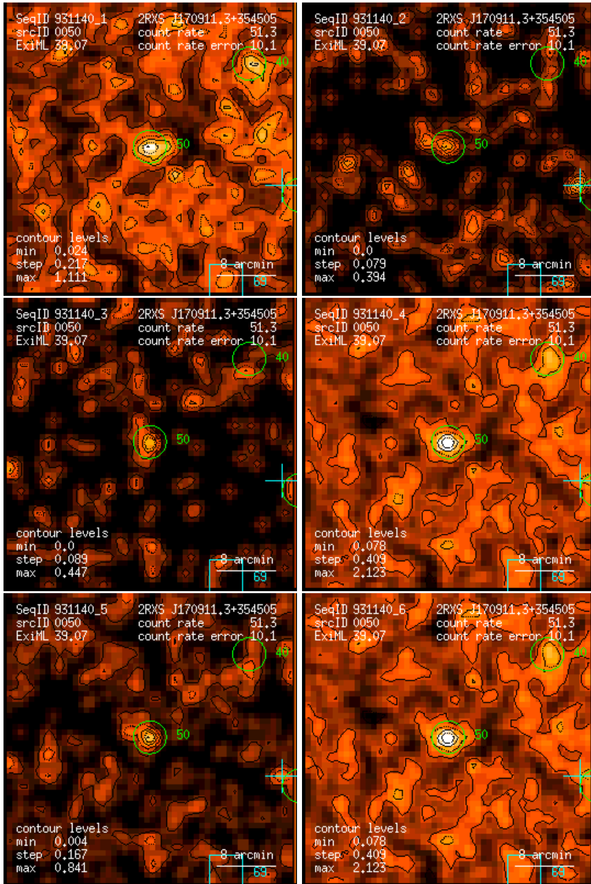
Figure 50: RASS 931140: detection 0050: band rate images, Gaussian filter: (1) PSPC channels 11 – 41, (2) 52 – 90, (3) 91 – 201, (4) 11 – 235, (5) 52 – 201, (6) 11 – 201. Broad band rates in counts/ks. Band rate contour levels in counts/ks/arcmin 2 .
