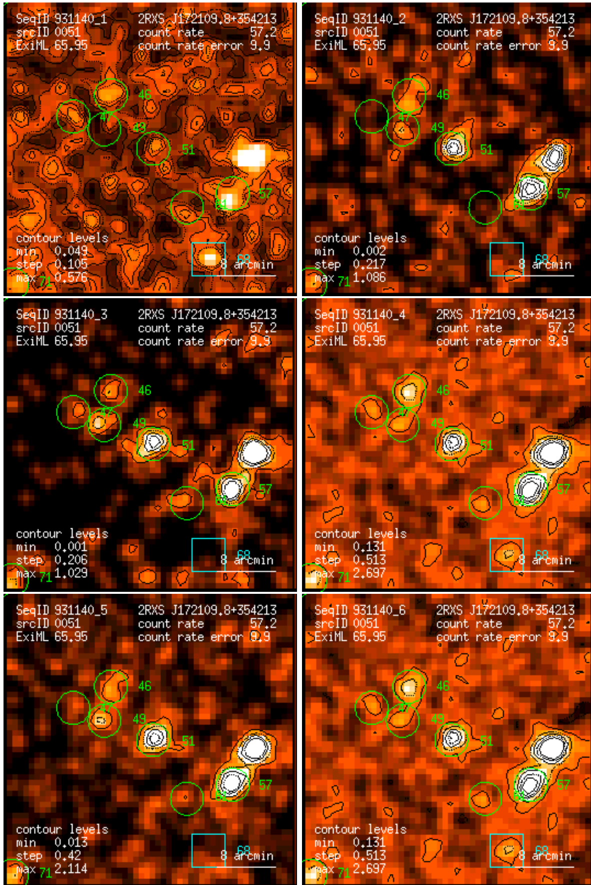
Figure 51: RASS 931140: detection 0051: band rate images, Gaussian filter: (1) PSPC channels 11 – 41, (2) 52 – 90, (3) 91 – 201, (4) 11 – 235, (5) 52 – 201, (6) 11 – 201. Broad band rates in counts/ks. Band rate contour levels in counts/ks/arcmin 2 .
