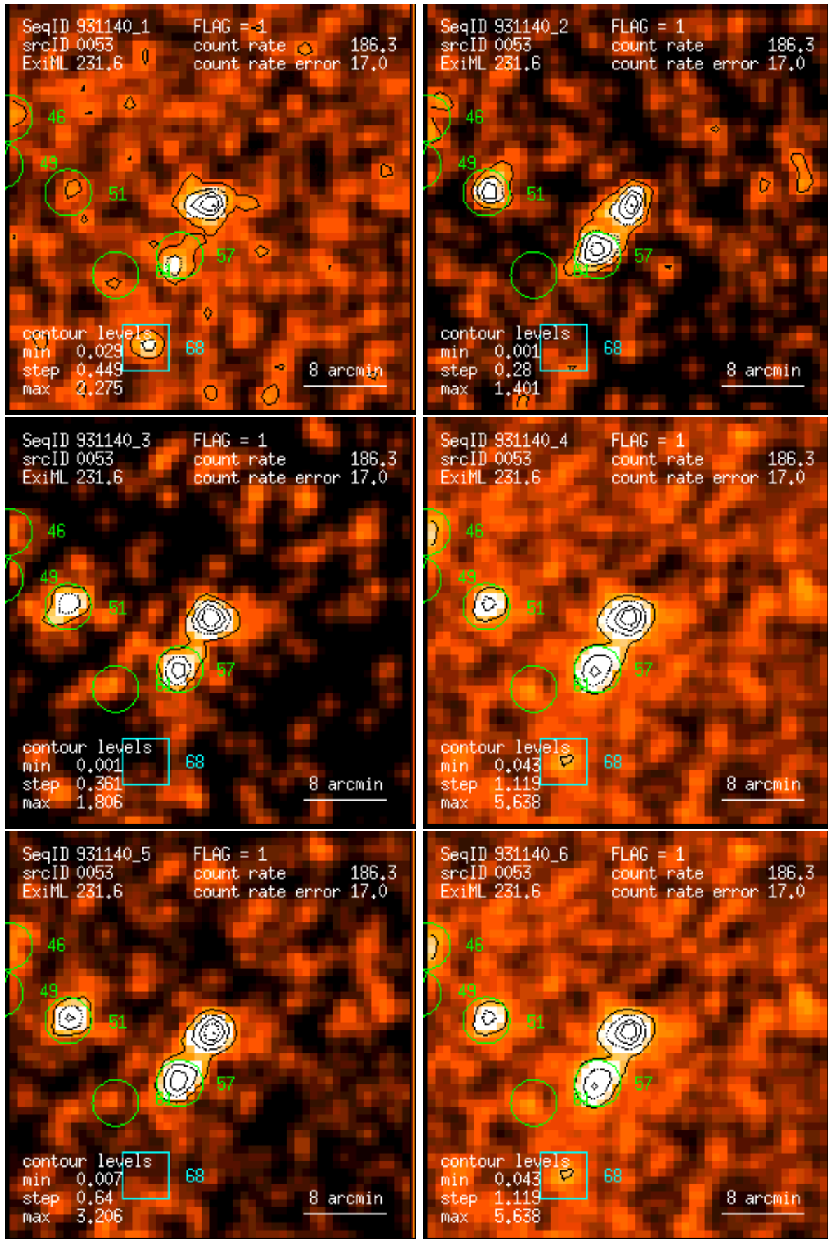
Figure 53: RASS 931140: detection 0053: band rate images, Gaussian filter: (1) PSPC channels 11 – 41, (2) 52 – 90, (3) 91 – 201, (4) 11 – 235, (5) 52 – 201, (6) 11 – 201. Broad band rates in counts/ks. Band rate contour levels in counts/ks/arcmin 2 .
