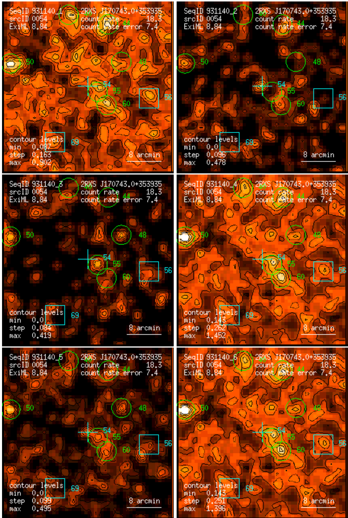
Figure 54: RASS 931140: detection 0054: band rate images, Gaussian filter: (1) PSPC channels 11 – 41, (2) 52 – 90, (3) 91 – 201, (4) 11 – 235, (5) 52 – 201, (6) 11 – 201. Broad band rates in counts/ks. Band rate contour levels in counts/ks/arcmin 2 .
