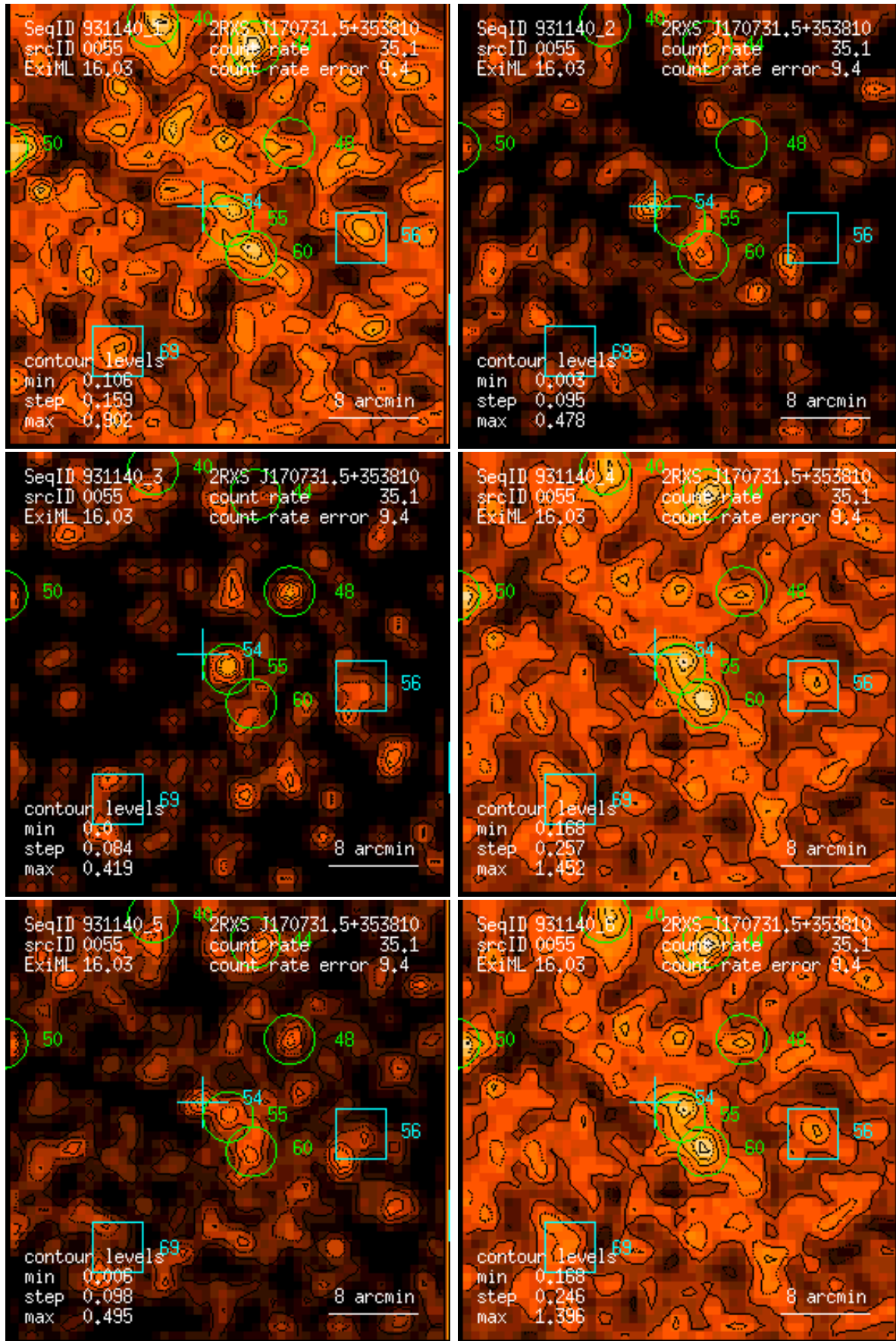
Figure 55: RASS 931140: detection 0055: band rate images, Gaussian filter: (1) PSPC channels 11 – 41, (2) 52 – 90, (3) 91 – 201, (4) 11 – 235, (5) 52 – 201, (6) 11 – 201. Broad band rates in counts/ks. Band rate contour levels in counts/ks/arcmin 2 .
