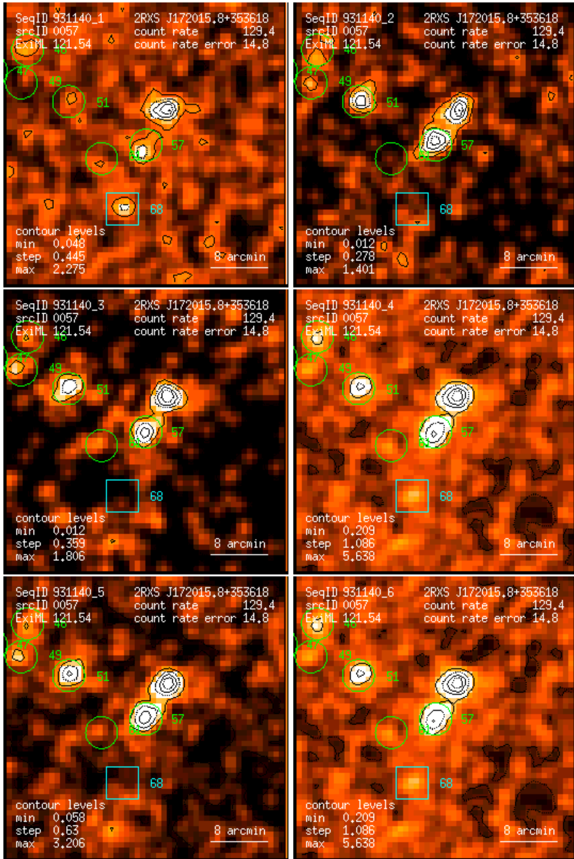
Figure 57: RASS 931140: detection 0057: band rate images, Gaussian filter: (1) PSPC channels 11 – 41, (2) 52 – 90, (3) 91 – 201, (4) 11 – 235, (5) 52 – 201, (6) 11 – 201. Broad band rates in counts/ks. Band rate contour levels in counts/ks/arcmin 2 .
